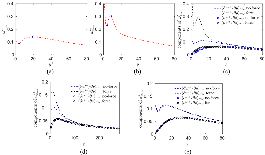
FIG. 10. Streamwise vorticity fluctuations. (a) Streamwise vorticity fluctuations, \omega_{x_{rms}}^+ , no-force case, Re_\tau = 180 . (b) Streamwise vorticity fluctuations, \omega_{x_{rms}}^+ , force case, Re_\tau = 180 . (c) The two terms of \omega_{x_{rms}}^+ . Re_\tau = 180 . (d) The two terms of \omega_{x_{rms}}^+ . Re_\tau = 550 . (e) The two terms of \omega_{x_{rms}}^+ for the discrete plasma areas with a spanwise spacing of z^+ = b^+ + 6 . Re_\tau = 180 .
