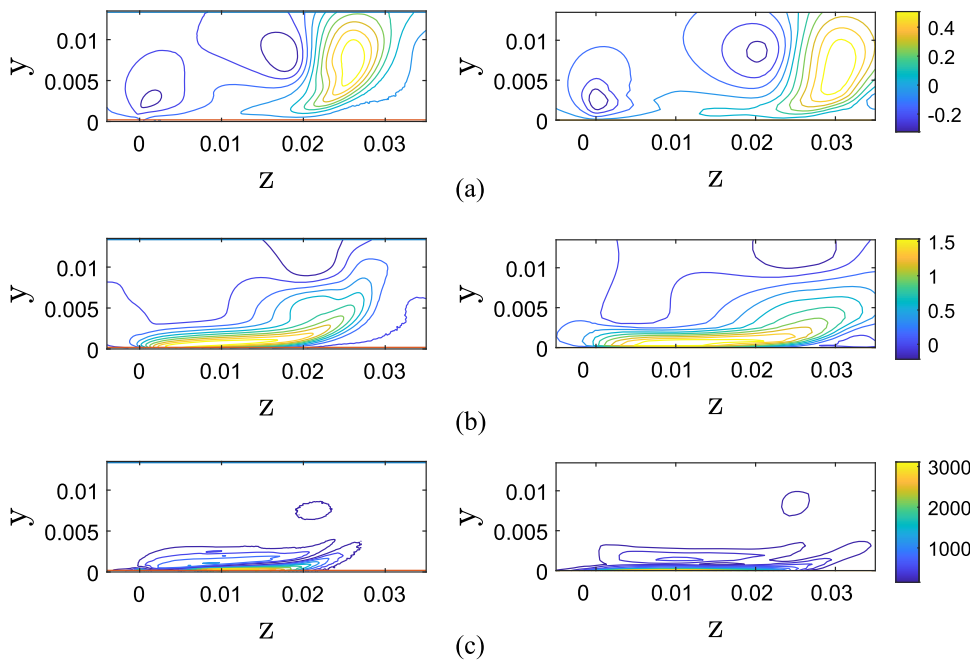
FIG. 3. (a) Wall-normal velocity, v , (b) plasma-aligned velocity, w , and (c) vorticity for the experimental study 3 in the left-hand side and numerical study in right-hand side.
