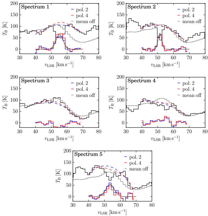
Fig. 6. Selected H I emission spectra corresponding the positions indicated in Fig. 1. The black lines represent the H I spectra, the colors correspond to the HISA. The gray spectra indicate the mean of the five off-positions presented in Fig. 5. The blue and red dashed lines represent the fits of the background to the HISA spectrum for a polynomial of second and fourth order, respectively, using the velocity range of v_{\text{LSR}} = 40\text{--}50 and 60\text{--}70 \text{km s}^{-1} for the baseline of the fit. The blue and red solid lines show the difference between fitted H I spectra and the measured H I spectra ( T_{\text{on-off}} in Eq. (4)) for a polynomial of second and fourth order, respectively. We fitted Spectra 1, 2, and 5 using a Gaussian function, shown by the black solid curve on top of the HISA spectra.
