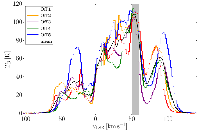
Fig. 5. Selected H I emission spectra around the GMF38a, which can be used as “off-positions”. The regions we used for the extraction are shown in Fig. 1. The black line shows the mean spectrum of all five off-spectra and the gray shaded area indicates the velocity range of the HISA feature ( v_{\text{LSR}} = 50\text{--}60 km s ^{-1} ).
