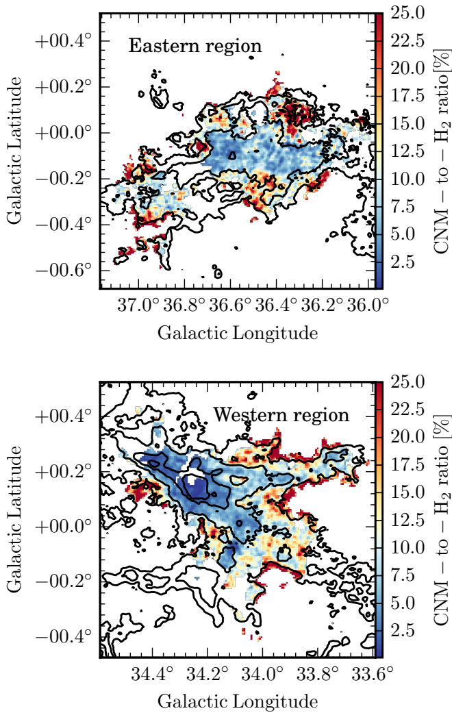
Fig. 15. Ratio of the CNM and H 2 column densities in percentage of the Eastern region ( top panel ) and Western region ( bottom panel ). The contours in both panels indicate the integrated 13 CO emission at levels of 5, 10, 20, and 30 K km s -1 .
