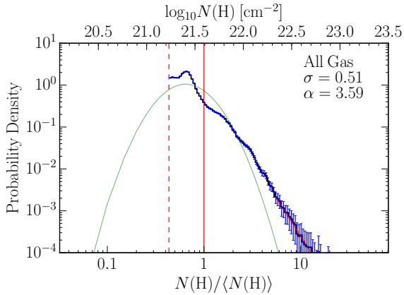
Fig. 21. N-PDF of the combination of atomic and molecular gas over the entire region in Fig. 14. The green line shows the log-normal fit. The dashed vertical line mark the column density threshold (the contour levels in Fig. 14), and the vertical solid line mark the mean column density. The red line shows the power-law fit with an index -\alpha to the high column density tail.
