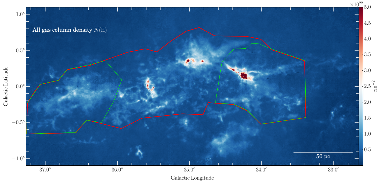
Fig. A.1. The column density map of the gas combined molecular component (from ^{13}\text{CO} ), CNM (from HISA), and WNM+CNM (from H I emission) (see Sect. 3.2.1). The red and green polygons mark the region for the mass estimates and the column density PDF measurements (only molecular component and CNM) shown in Figs. 20 and 22, respectively.
