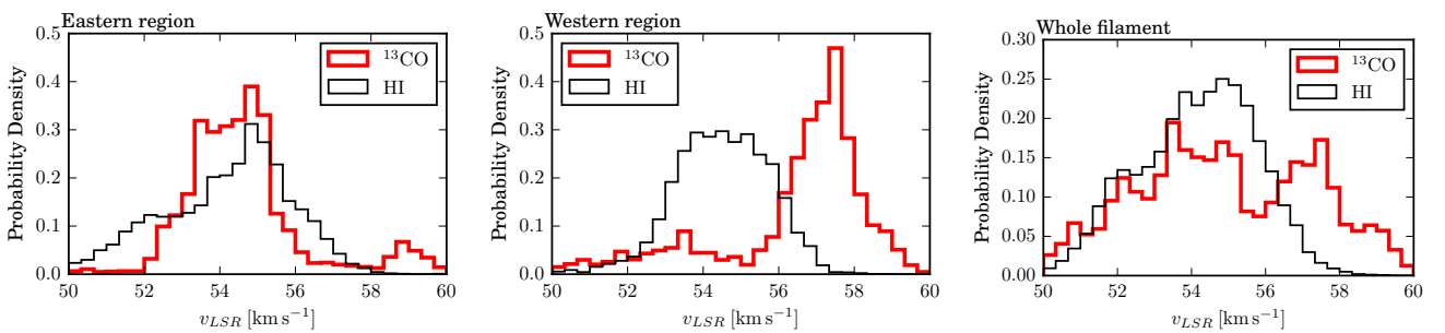
Fig. 10. Histograms of the HISA and ^{13}\text{CO} peak velocity, shown in black (thin) and red (thick) respectively. Left and middle panels : all extracted pixels within the marked eastern (around l = 36.5^\circ ) and western (around l = 34^\circ ) polygon in Fig. 14. Right panel : all extracted pixels for the whole filament (red polygon in Fig. 14).
