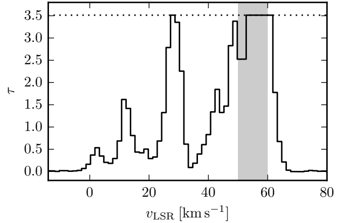
Fig. 18. Spectrum of the H I optical depth towards the UCH II region G34.256+0.146 using the THOR data. For some channels, the absorption spectra saturates and the measured optical depth is a lower limit of \tau = 3.5 , which is indicated by the dotted line. The gray shaded area indicates the velocity range of the HISA feature ( v_{\text{LSR}} = 50\text{--}60 \text{ km s}^{-1} ).
