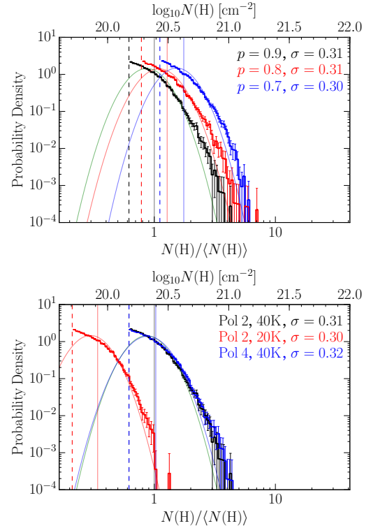
Fig. 23. Top panel: N-PDFs for the atomic hydrogen for different p . The PDF is measured over the entire filament indicated with a red polygon in Fig. 14, assuming a constant spin temperature of T_{\text{HISA}} = 40 \text{ K} . Bottom panel: N-PDFs for the atomic hydrogen for different spin temperature and different polynomial functions fit to get T_{\text{off}} . The dashed vertical lines in each panel indicate the column density threshold, and the solid vertical lines indicate the mean column densities. The bottom x-axes in both panels are the relative column densities for the N-PDF of “Pol 2, p=0.9, 40 \text{ K} ”, i.e., the black histogram in both panels. Other N-PDFs are shifted to the correct absolute column density for comparison.
