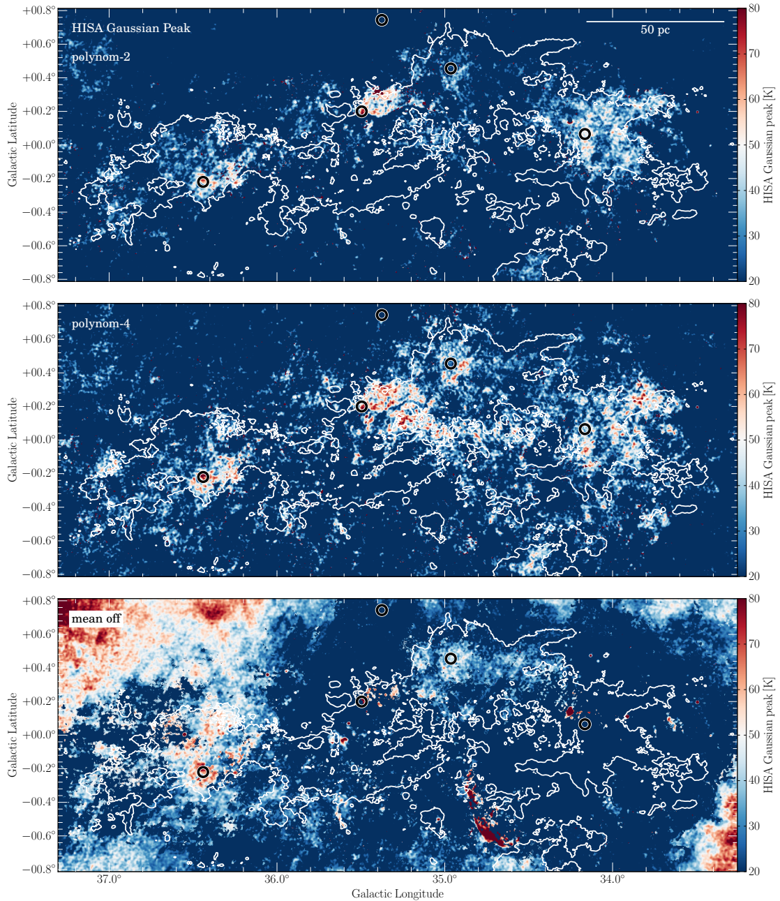
Fig. 7. Peak value of a Gaussian fit for the absorption depth T_{\text{off}} - T_{\text{on}} for different methods of estimating T_{\text{off}} . Top and middle panels: method using a polynomial fits with second and fourth order, respectively. Bottom panel: method using a spatially averaged off spectrum shown in Fig. 5. The white contours represent the integrated ^{13}\text{CO} emission at levels of 5 \text{ K km s}^{-1} for reference. The circles from left to right marked the same positions as in Fig. 1 where Spectra 1 to 5 shown in Fig. 6 are extracted, respectively.
