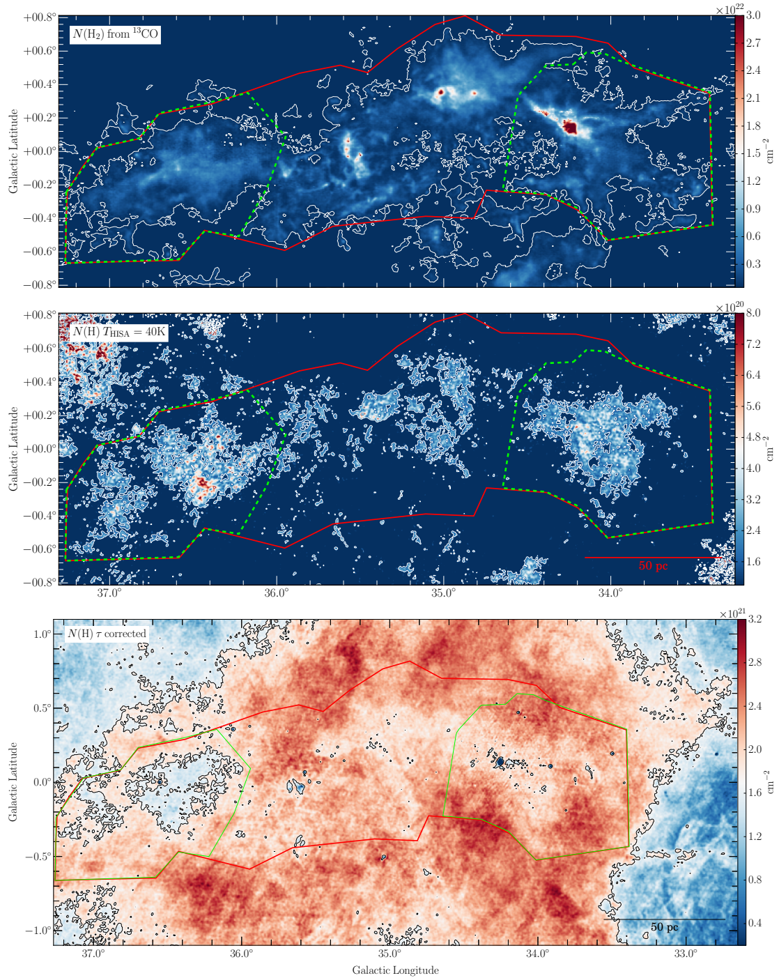
Fig. 14. Top panel: column density map of the molecular cloud derived from ^{13}\text{CO} emission (see Sect. 3.2.1). Middle panel: column density map of the CNM derived from HISA, assuming T_S = 40\text{ K} , p = 0.9 and using a second order polynomial to estimate the background temperature T_{\text{off}} . Bottom panel: optical depth corrected column density map of atomic hydrogen derived from H I emission. The contours indicate column density threshold used for the N-PDFs (see Sect. 4.5). For the \text{H}_2 , HISA, and H I emission they have levels of 6 \times 10^{20} , 1.5 \times 10^{20} , and 1.7 \times 10^{21}\text{ cm}^{-2} , respectively. The red and green polygons mark the region for the mass estimates and the column density PDF measurements shown in Figs. 20 and 22, respectively.
