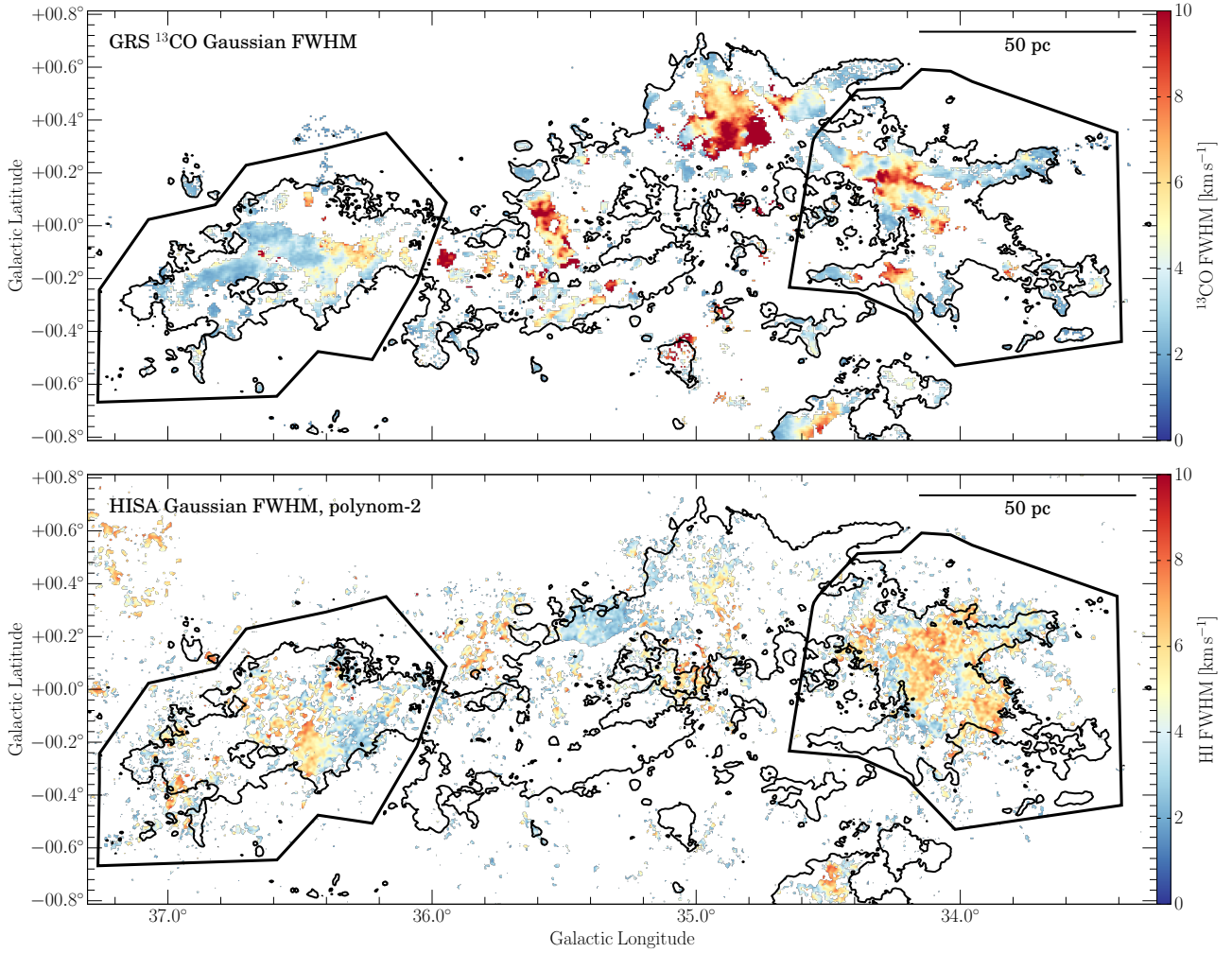
Fig. 11. Full width at half maximum (FWHM) of the ^{13}\text{CO} emission ( top panel ) and the HISA feature ( bottom panel ), respectively. The linewidth is determined by using a single Gaussian fit. The contours indicate the integrated ^{13}\text{CO} emission at levels of 5 \text{ K km s}^{-1} for reference. The polygons mark the eastern (around l = 36.5^\circ ) and western (around l = 34^\circ ) subregions, for which we present the histograms of the FWHM linewidths in Fig. 12.
