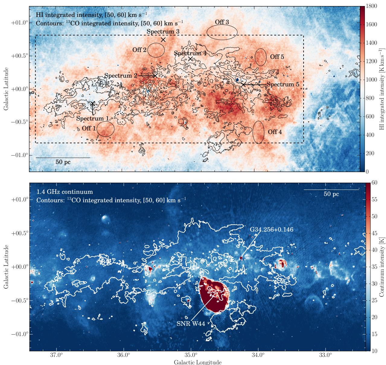
Fig. 1. Overview of the giant molecular filament GMF38a. Top panel: ^{13}\text{CO} (GRS, Jackson et al. 2006) integrated intensity contours in the range v_{\text{LSR}} = 50\text{--}60\text{ km s}^{-1} overlaid on integrated HI emission in the same velocity range. The black ellipses show the “off-positions” whose spectra are shown in Fig. 5 and the black “x” signs mark positions whose spectra are shown in Fig. 6. Bottom panel: same ^{13}\text{CO} integrated intensity contours overlaid on 1.4 GHz continuum emission from the THOR survey (Wang et al. 2018). The contours in the top panel indicate integrated ^{13}\text{CO} emission levels of 5, 10, 20, and 30 \text{K km s}^{-1} . The contours in the bottom panel indicate integrated ^{13}\text{CO} emission levels of 5 \text{K km s}^{-1} for reference. The dashed box in the top panel outlines the region that is discussed in the following sections and shown in Figs. 7, 9, 11, 14, and 19.
