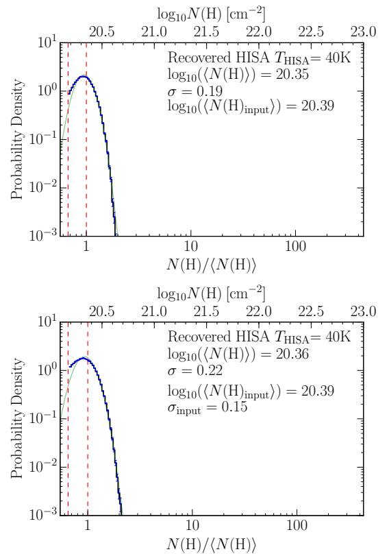
Fig. B.1. The N-PDFs of the CNM recovered from the tests.
