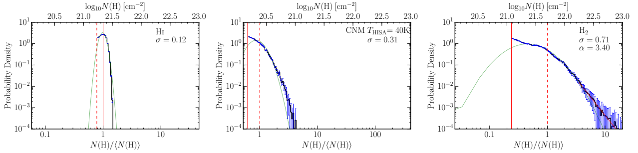
Fig. 20. N-PDFs of the gas traced by H I ( left panel ) emission, HISA ( middle panel ), and ^{13}\text{CO} ( right panel ) in units of hydrogen atoms per square cm. The light green lines show the log-normal fit in each panel. \sigma is the width of the log-normal distribution. The dashed vertical lines in each panel mark the column density threshold, and the solid vertical lines mark the mean column densities. The red line in the ^{13}\text{CO} panel shows the power-law fit with an index -\alpha to the high column density tail.
