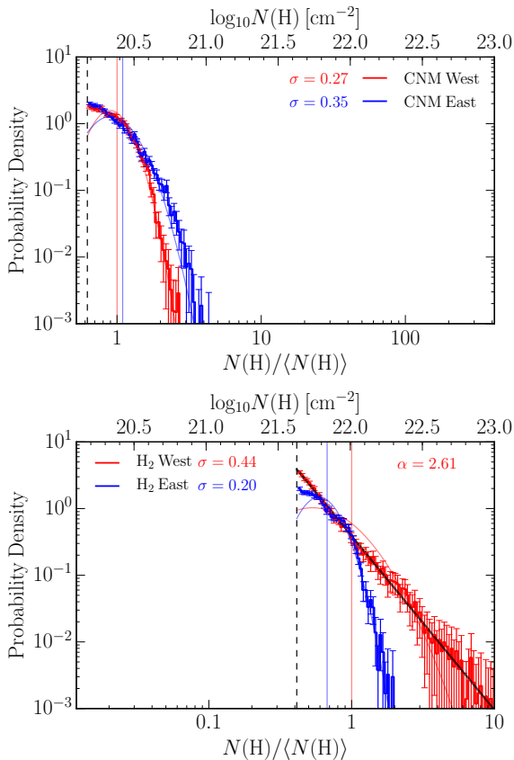
Fig. 22. N-PDFs for the two subregions within the filament marked with dashed polygons in Fig. 14. Top and bottom panels: N-PDF of atomic and molecular hydrogen derived with HISA and ^{13}\text{CO} measurements, respectively. The lighter lines show the log-normal ( top and bottom panels ) and power-law ( bottom panel ) fits. The black dashed lines in each panel mark the column density threshold, and the solid vertical lines indicate the mean column densities. The bottom x -axes in both panels are the relative column density for the N-PDF of the western subregion, i.e., the red histogram in both panels. Other N-PDFs are shifted to the correct absolute column density for comparison. The thick black line in the molecular component panel shows the power-law fit with an index -\alpha to the column density distribution of the western region.
