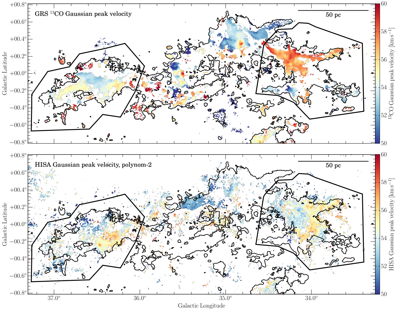
Fig. 9. Peak velocity of the Gaussian fit of the ^{13}\text{CO} data ( top panel ) and the HISA data ( bottom panel ), respectively. The HISA are extracted by using a second order polynomial to estimate the background emission. The black contours indicate the integrated ^{13}\text{CO} emission at levels of 5 \text{ K km s}^{-1} . The polygons mark the eastern (around l = 36.5^\circ ) and western (around l = 34^\circ ) subregions, for which we present the histograms of the peak velocities in Fig. 10.
