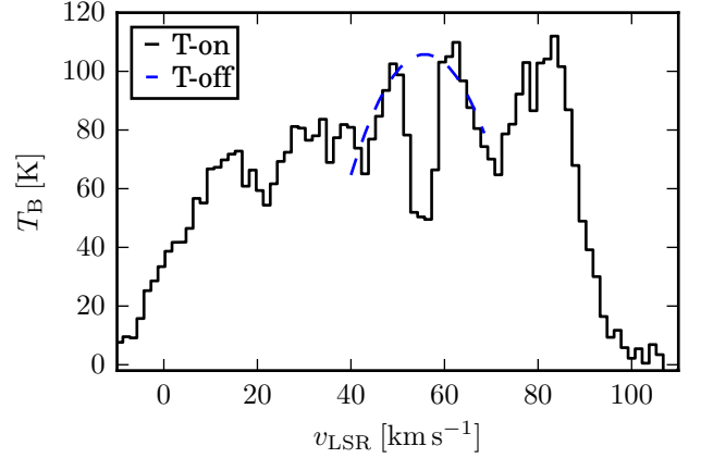
Fig. 3. Sample spectrum showing a prominent HISA feature around v_{\text{LSR}} \sim 55 \text{ km s}^{-1} . The actual HI spectra is shown in black ( T_{\text{on}} ) and the estimated background emission using a second order polynomial fit (see Sect. 2.3) is shown in blue ( T_{\text{off}} ).
