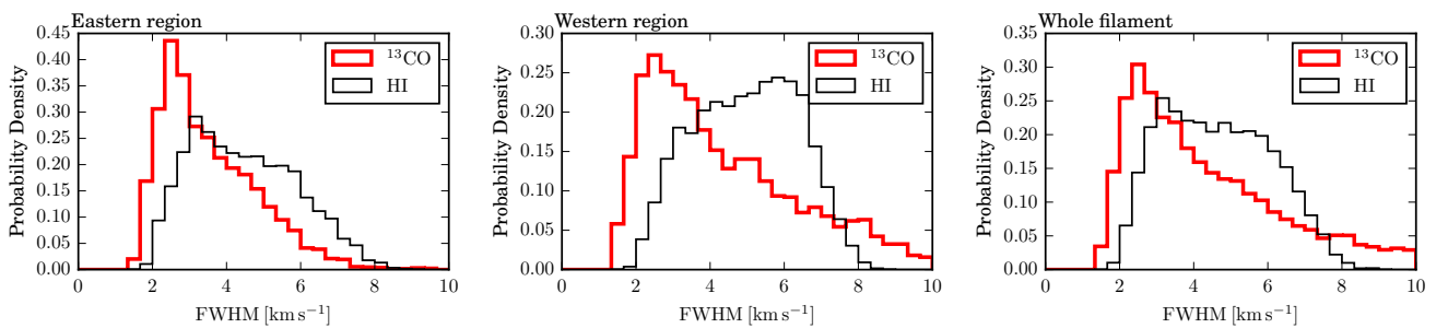
Fig. 12. Histograms of the FWHM linewidth of the HISA and ^{13}\text{CO} emission in black (thin) and red (thick), respectively. Left and middle panels: all extracted pixels within the marked eastern (around l = 36.5^\circ ) and western (around l = 34^\circ ) polygon in Fig. 14. Right panel: all extracted pixels for the whole filament (red polygon in Fig. 14).
