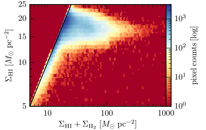
Fig. 16. Surface density of the atomic hydrogen ( v_{\text{lsr}} = 50\text{--}60 km s -1 ) as a function of the total gas surface density ( \Sigma_{\text{HI}} + \Sigma_{\text{H}_2} ). The solid line represents a one-to-one relation.
