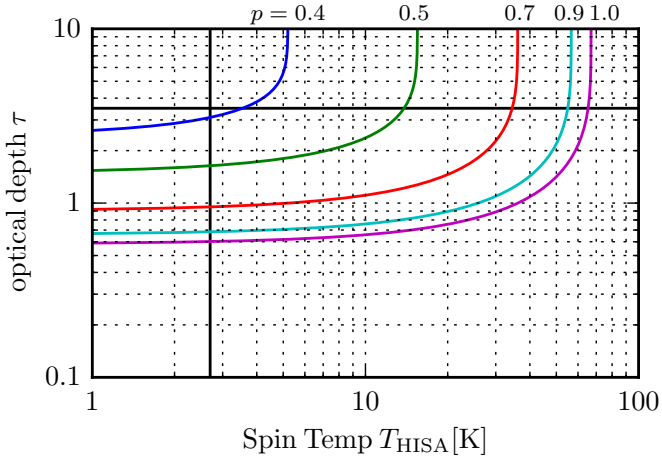
Fig. 4. Optical depth as a function of the spin temperature (as introduced in Eq. (4)) for the region close to the strong continuum source G34.256+0.146 with T_{\text{off}} = 103 K, T_{\text{on}} = 50 K, and T_{\text{cont}} = 17 K. The optical depth of \tau = 3.5 is indicated with a black horizontal line. The temperature of the CMB is indicated at T = 2.7 K with a black vertical line.
