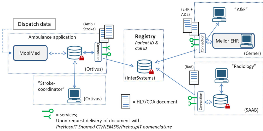
Fig. 1 PrehospIT system design
