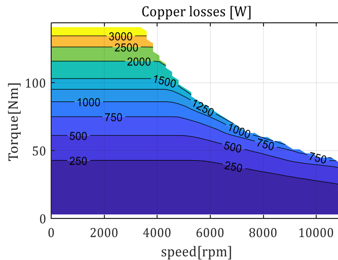
Figure A1. Copper loss map from FEA.
