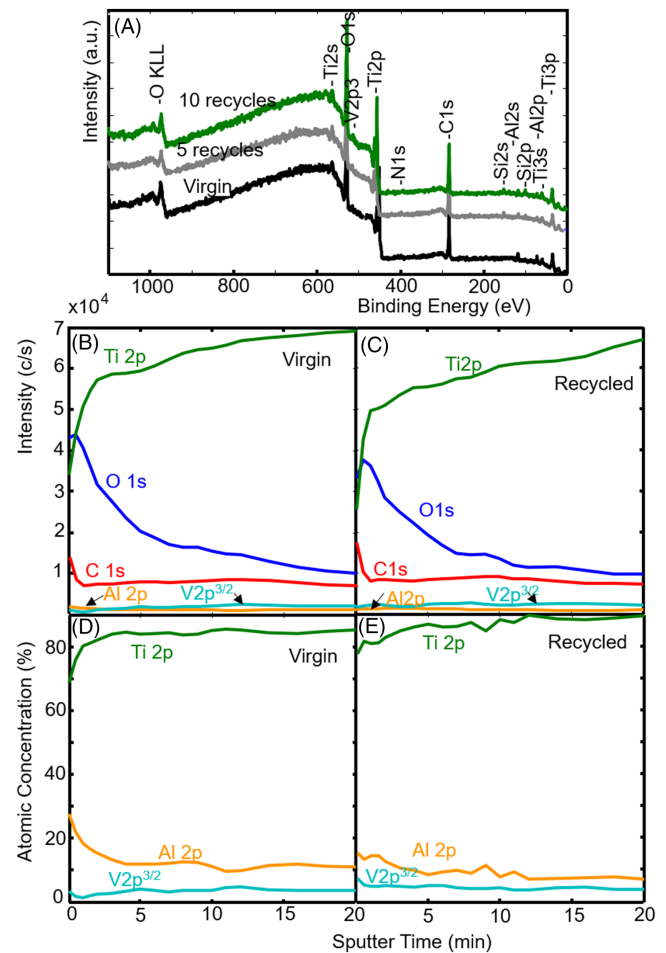
FIGURE 2 X-ray photoelectron spectroscopy survey spectra from the powders (A); X-ray photoelectron spectroscopy depth profiles (B, C) and cation profiles (D, E) from virgin powder (B, D) and powders recycled for 5 times (C, E). The etch rate is 24.8 \text{\AA}/\text{min} for \text{Ta}_2\text{O}_5 with known oxide thickness
