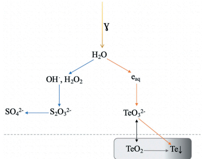
Fig. 7. Schematic presentation of the system with \text{TeO}_2 as the precursor in ABS with the sodium thiosulfate.
