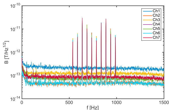
Fig. 3. Spectrum of the measured magnetic fields showing peaks at the coil signal frequencies.
