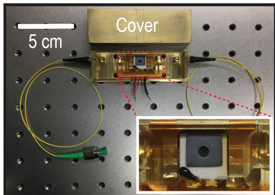
Fig. 1. Packaged micro-comb device.
