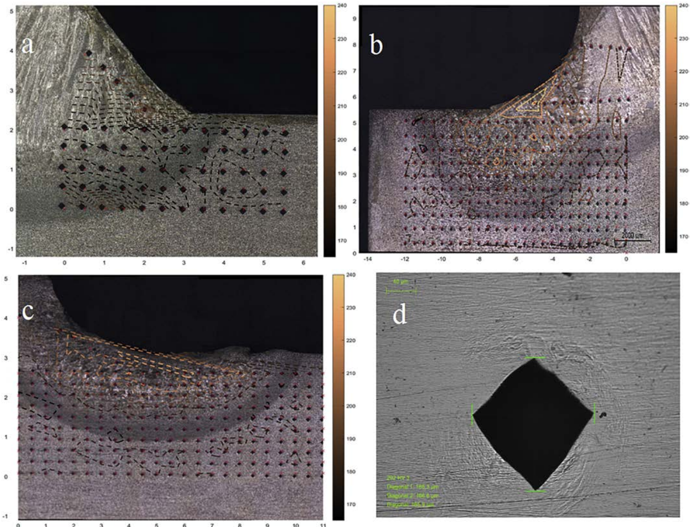
Fig. 10. The hardness distribution in the vicinity of the weld in: a: as-welded b: TIG-treated c: TIG-HFMI treated d: Vicker's hardness indent sample.
