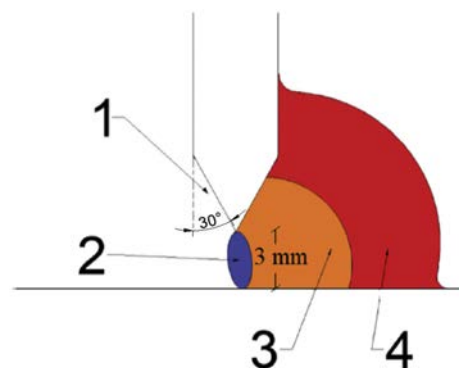
Fig. 2. Welding procedures: 1: Machining the stiffener. 2: Tack welding. 3: Root welding. 4: Cap welding.
