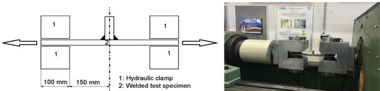
Fig. 4. L: Schematic figure shows the hydraulic clamp. R: Fatigue testing rig.
