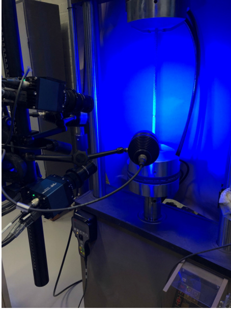
Fig. 3. DIC setup for the tensile test.
