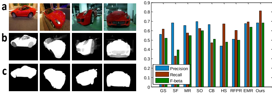
Figure 3.18: Performance of the proposed co-saliency detection method on iCoseg dataset. Left: performance on one set of images, (a) original images; (b) the proposed; and (c) ground truth. Right: comparison with eight saliency detection models on weighed precision, recall and F-beta.
