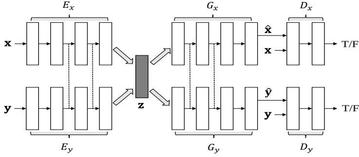
Figure 2.7: Illustration of unsupervised image-to-image translation [110] using shared latent space assumption. A pair of images (x, y) are mapped to the same latent code z using two encoding functions E_x and E_y , followed by two generators G_x and G_y to map the latent code to images. D_x and D_y are two corresponding discriminators.
