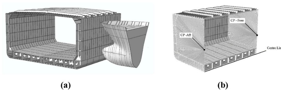
Fig. 3. (a) Definition of collision scenario with positioning of the two vessels. Note that the bulb hits the bilge area and the forecastle on the shear strake. (b) Constrained FE model of the struck vessel showing the CPs.
