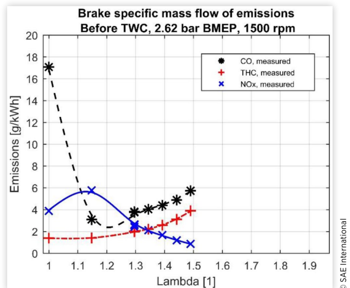
FIGURE 17 Engine out CO, THC and NO x emissions as brake specific mass flow, plotted vs lambda at 2.62 bar BMEP and 1500 rpm. Three repetitions included at lambda 1.3. All corresponding lines are fitted spline-curves.
