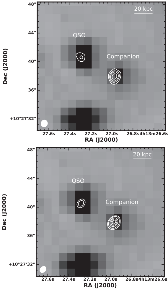
Figure 1. ALMA 150 GHz ( upper panel ) and 240 GHz ( lower panel ) dust continuum contours overlaid on the Spitzer IRAC 4.5 \mu\text{m} image of SMM J04135+10277. The beam size is indicated in the bottom left corner. The contour levels are 5\sigma , 10\sigma , 15\sigma , 25\sigma for the 150 GHz continuum and 25\sigma , 50\sigma , 75\sigma , 100\sigma for the 240 GHz continuum.
