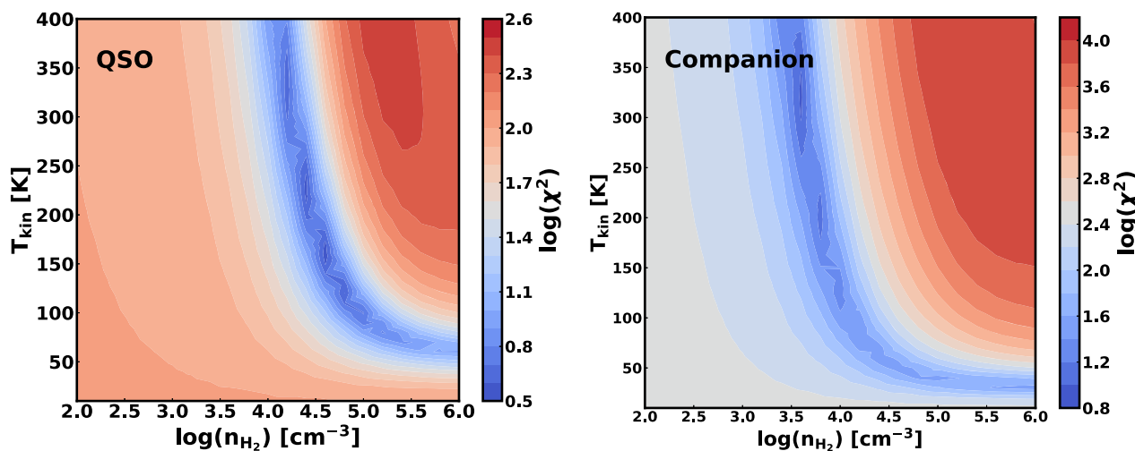
Figure 6. \chi^2 contour plots of SMM J04135+10277. The contour plots trace the \chi^2 value of the RADEX CO models as a function of molecular hydrogen density and temperature. The left-hand panel shows the fitting results of the quasar and the right-hand panels shows the same for the companion galaxy.
