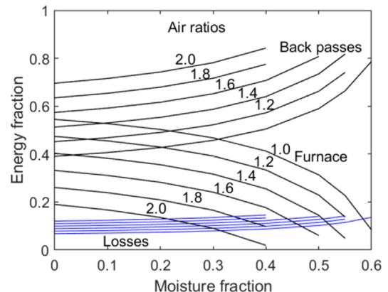
Fig. 8. The fractions of energy recovered in the furnace, in the back passes, and losses with the off-gas from the stack. The exit temperature from the furnace was put to 900 °C and the flue gas temperature in the off-gas 150 °C. The losses (the lower curves) are largest at a high excess air.
