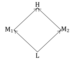
Figure 3: Lattice \langle \mathcal{L}_\circ, \sqsubseteq \rangle
