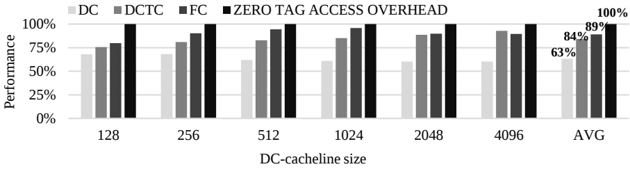
Figure 2.1: Performance normalized to DRAM cache without tag access overhead. The depicted results are the average performance results retrieved for the SPEC and NAS benchmarks used in our evaluation section.
