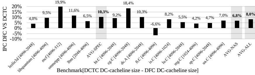
(b) DFC performance improvement compared to DCTC at best DC-cacheline size
