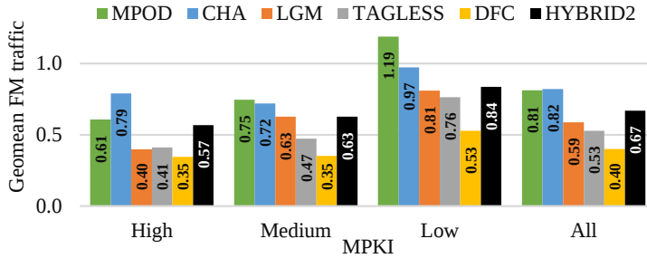
Figure 4.16: Geometric mean of normalized FM traffic for benchmarks with high, medium, and low MPKI.
