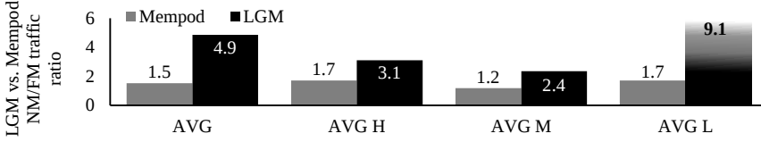
Figure 3.11: NM to FM processor request ratio of MempoD and LGM.
