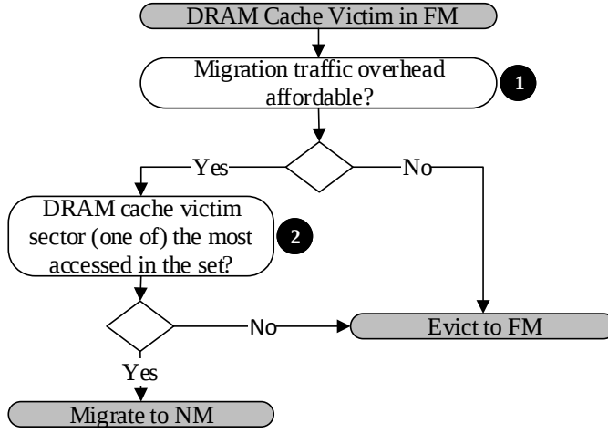
Figure 4.10: Migration decision.
