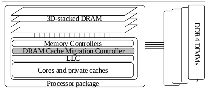
Figure 4.3: System Overview.
