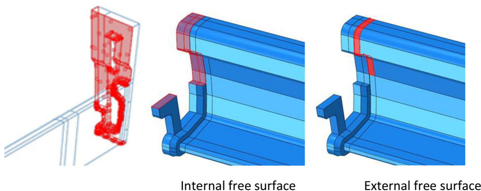
Fig. 3 Left, convective surfaces; highlighted in red, model the heat transfer between the weld metal and mold; mid and right, new free surfaces and convective boundaries after material has been removed by a shearing device
