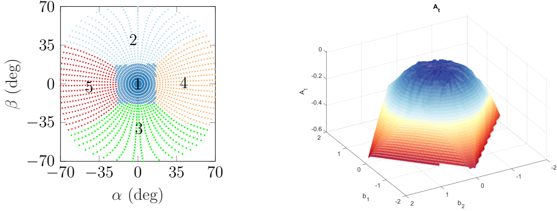
(a) Local interpolation scheme, each sector is marked with the highest pressure perceiving port (b) Total Pressure coefficient A_t in sector one
