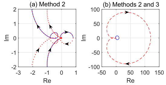
Fig. 8. Example 1: Nyquist curves for \alpha_d = \alpha_p = 0.4 p.u. (a) \lambda(j\omega) (solid) and characteristic loci of \mathbf{G}(j\omega) (dotted). (b) \lambda(j\omega) (solid) and \gamma(j\omega) (dashed).
