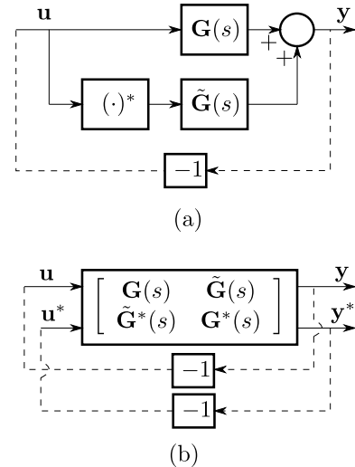
Fig. 1. (a) Asymmetric complex space-vector SISO model. (b) Corresponding MIMO model. The dashed lines show optional feedback loops that are considered in Section III.
