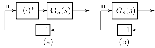
Fig. 4. (a) Antisymmetric outer loop with \mathbf{G}_a(s) = \tilde{\mathbf{G}}(s)\mathbf{S}(s) . (b) Equivalent symmetric outer loop with G_s(s) = -\mathbf{G}_a(s)\mathbf{G}_a^*(s) .
