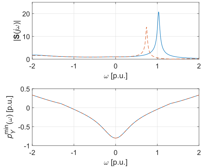
Fig. 12. Example 3: sensitivity function and input-admittance passivity index for \omega_{res} = 5.0 p.u. (solid) and \omega_{res} = 2.36 p.u. (dashed).
