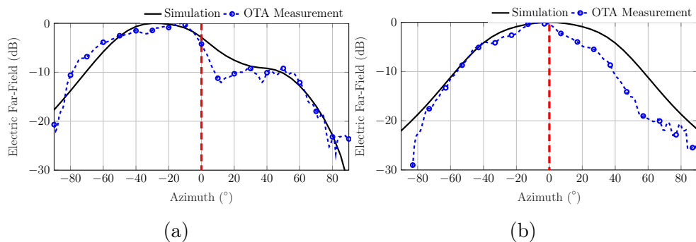
Figure 4.7: H-plane radiation pattern ( El = 0^\circ ) versus steered angle: a) (Az_s, El_s) = (-30^\circ, 0^\circ) , b) (Az_s, El_s) = (0^\circ, 0^\circ) , The red dashed line shows the boresight angle.
