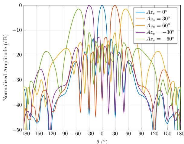
Figure 2.3: Radiation pattern of an 8 \times 8 microstrip patch antenna array in the El_s = 0 (x-z) plane. The steer angles are El_s = 0 ; Az_s = -60^\circ, -30^\circ, 0^\circ, 30^\circ, 60^\circ .
