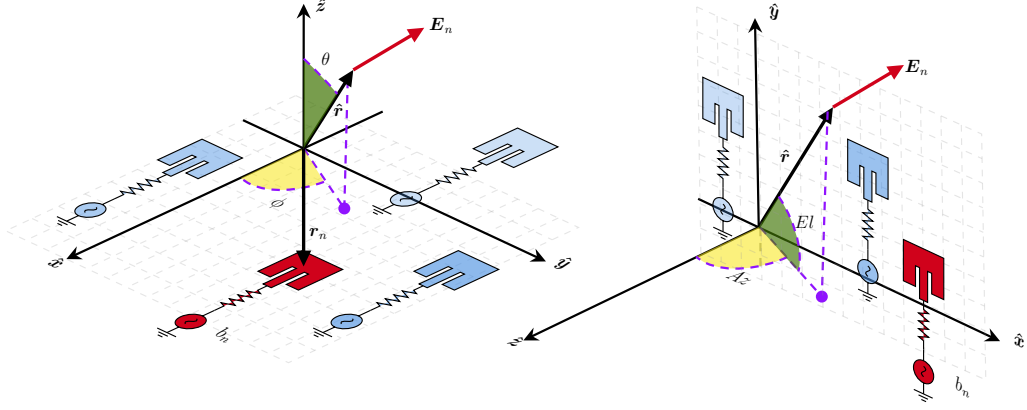
Figure 2.1: Illustration of a generic antenna array layout in spherical coordinate system (left) and Azimuth/Elevation coordinate system (right); each antenna element is located in position \mathbf{r}_n . The element radiated field is \mathbf{E}_n , and excitation waves are b_n .
