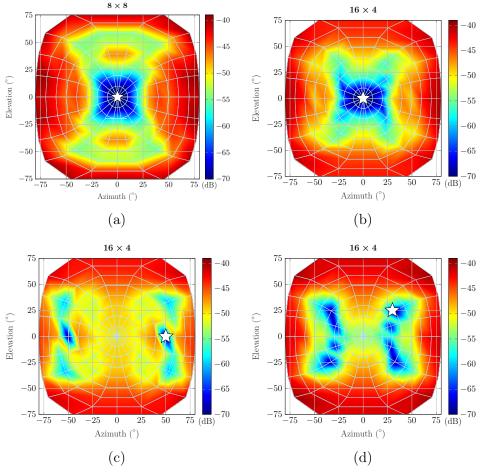
Figure 4.9: Nonlinear distortion in the far-field versus steering angle for a) 8 \times 8 array linearized for the beam at (Az_t, El_t) = (0, 0)^\circ , b) 16 \times 4 array linearized for (Az_t, El_t) = (0, 0)^\circ , c) 16 \times 4 array linearized for (Az_t, El_t) = (50, 0)^\circ , and d) 16 \times 4 array linearized for (Az_t, El_t) = (30, 25)^\circ . The results are presented in terms of normalized mean square error for an LTE signal with 8.5 peak-to-average power ratio. The white filled star represents the direction that the beam-dependent DPD is optimized for.
