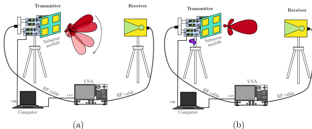
Figure 4.5: Block diagram of the setup for a) far-field signal distortion measurement, b) radiation pattern measurement.
