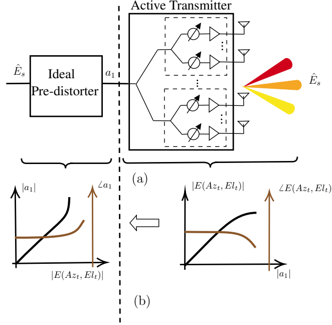
Figure 4.8: a) Structure of hybrid beamforming transmitter utilizing an ideal predistorter. b) The conceptual representation of the transmitter transfer AM/AM and AM/PM function and corresponding pre-distorter.
