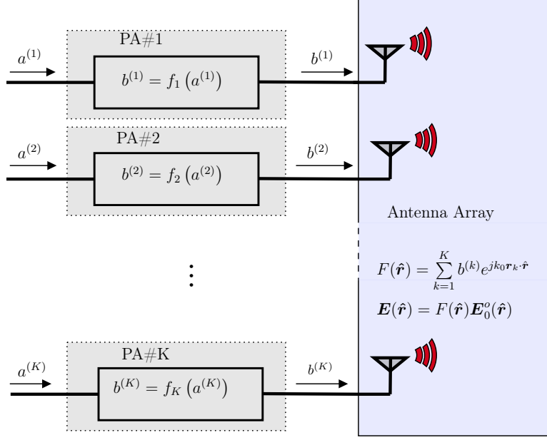
Figure 4.1: The modeling framework of active transmitter antenna array with isolated RF transmit paths
