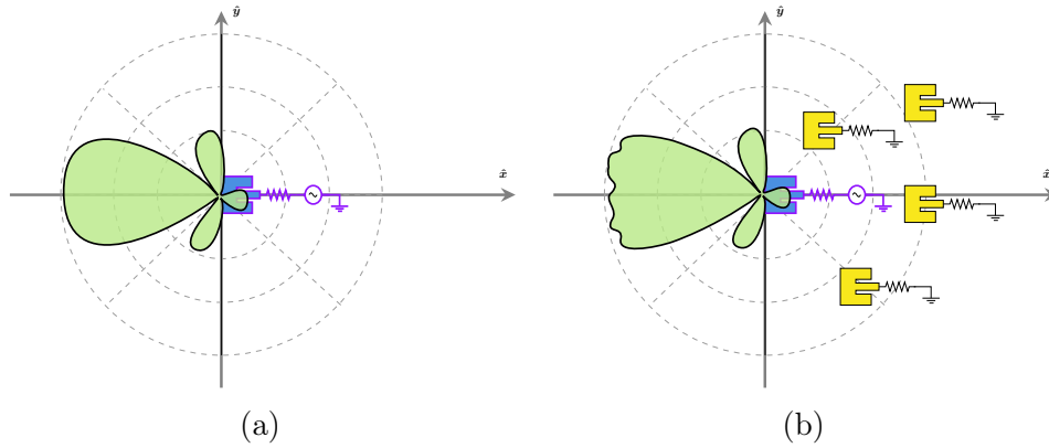
Figure 2.4: The antenna element radiation pattern. a) Isolated element pattern, b) Embedded element pattern; For a weakly coupled array, the isolated element pattern and embedded element pattern become similar.
