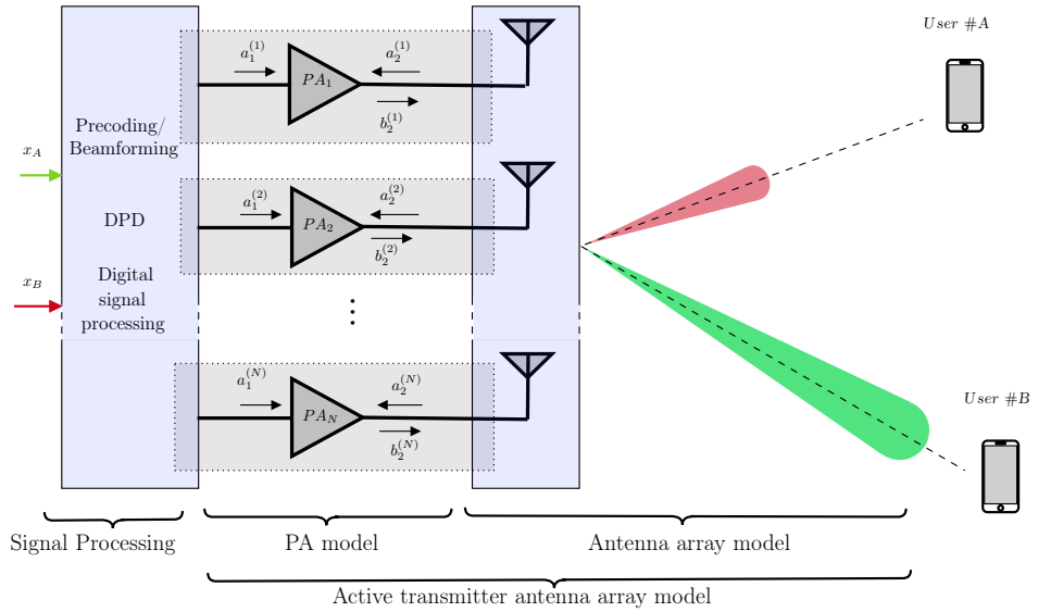
Figure 1.3: The analysis framework for an active transmitter antenna array.
