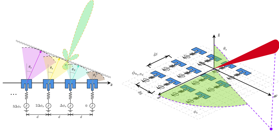
Figure 2.2: Illustration of a linear (left) and planar (right) phased array; \Delta\phi_x is phase shift in linear array. N_x and N_y are the number of elements in planar array along x and y axis, respectively. \phi_{n_x, n_y} is the excitation phase of corresponding element.
