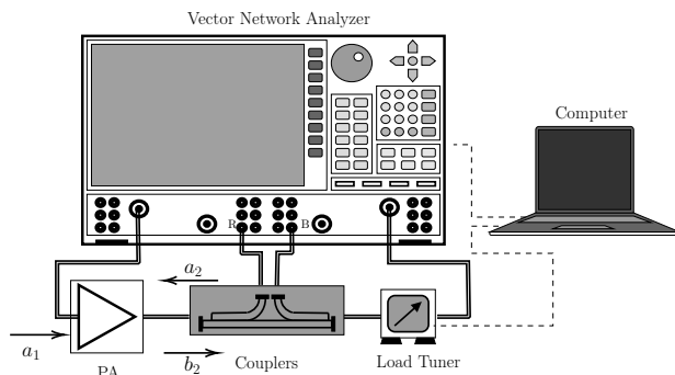
Figure 3.3: Block diagram of a conventional load-pull measurement setup.
