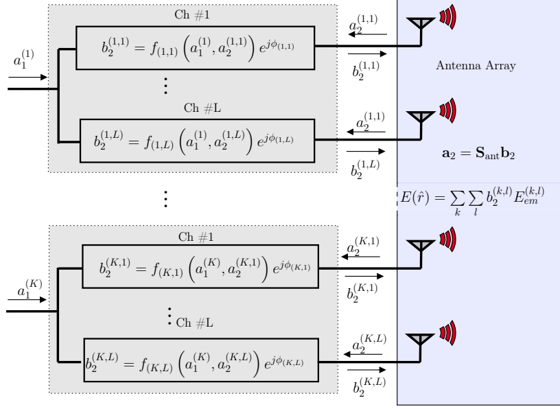
Figure 4.3: The modeling framework for a hybrid beamforming transmitter.
