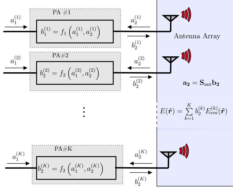
Figure 4.2: The modeling framework for active transmitter antenna array with non-negligible antenna array mutual coupling.
