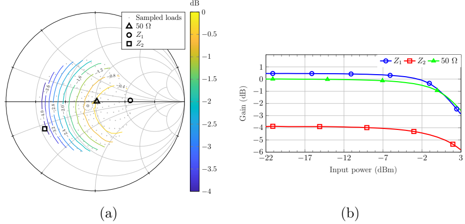
Figure 3.4: a) Normalized delivered output power contours from load-pull measurement at 29 GHz. Markers are Z_1 = 115 + j4 , Z_2 = 11 - j12 and 50\Omega . Gray points indicate loads used during load-pull characterization, b) Normalized AM/AM for the different marked loads Z_1 , Z_2 and 50\Omega . The results are normalized to the small signal measurements with a 50\Omega load.
