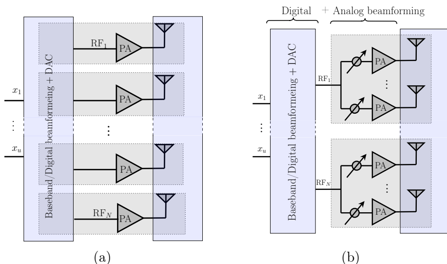
Figure 1.2: Different architectures for a transmitter in a MIMO system. a) Digital beamforming, b) Hybrid digital and analog beamforming architecture.
