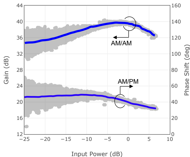
Figure 3.1: An example of PA AM/AM and AM/PM characteristics. Dispersive gray dots show dynamic PA behavior under modulated input signal with 10 MHz bandwidth [20].
