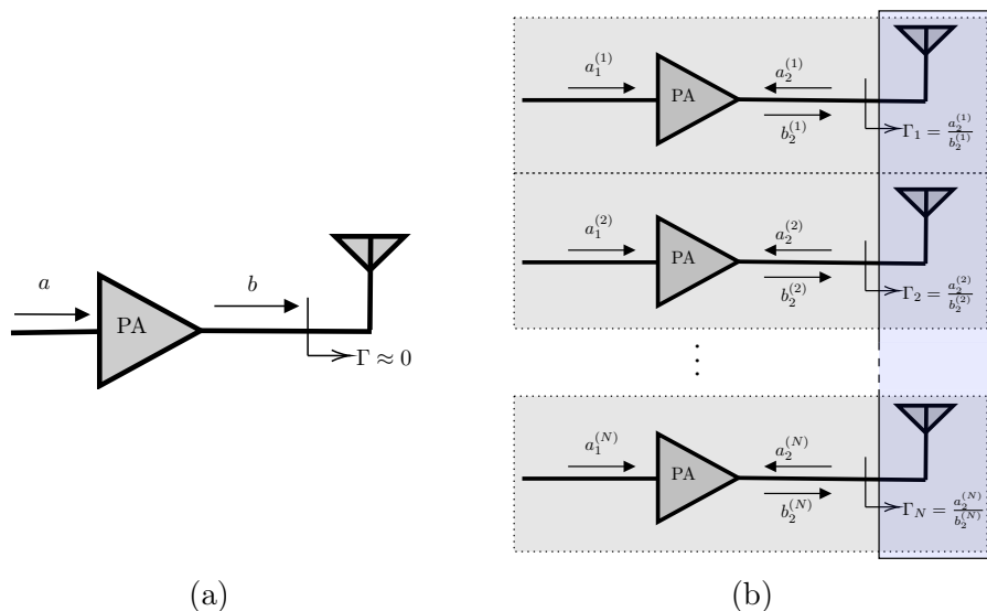
Figure 3.2: Block diagram of a) single path, b) multi path transmitter for the purpose of PA modeling
