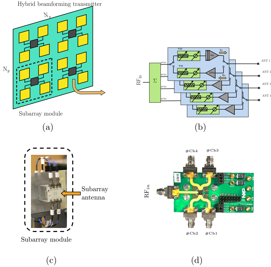
Figure 4.4: Hybrid beamforming transmitter and its building blocks. a) Subarray module, b) Beamforming IC block diagram, c) Picture of implemented subarray module, d) Evaluation board of the quad channel beamforming IC.
