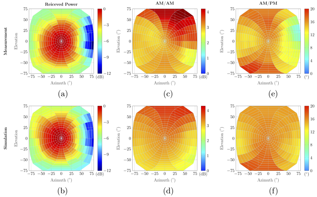
Figure 4.6: Normalized received power together with amplitude and phase compression variation in the far-field for different azimuth and elevation steering angles, |Az_s| < 80^\circ , |El_s| < 75^\circ . Normalized received power: a) OTA experiment b) Simulation. Amplitude compression: c) OTA experiment d) Simulation. Phase compression: e) OTA experiment f) Simulation. The RMS error between simulation and measurement of the amplitude and phase compression is 0.18 dB and 1.6 degrees, respectively.
