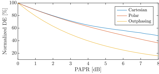
Figure 2.11: Modulation dependent DE as a function of PAPR, plotted for Cartesian, polar and outphasing transmitters. The DE is normalized to the peak for each individual transmitter topology.
