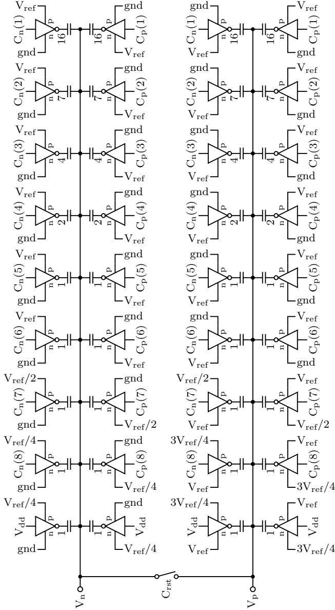
Figure 5.3: Schematic representation of the double balanced CDAC. The number of parallel unit cells in each stage is highlighted by the number next to the cell.
