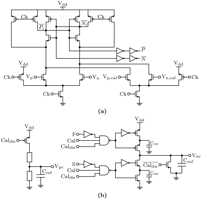
Figure 5.2: Schematic of the strong-ARM comparator used (a) and the calibration circuitry used for reducing effects of comparator offset voltage (b).
