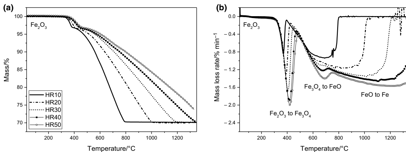
Fig. 1 TG/DTG curves of reduction of \text{Fe}_2\text{O}_3 reference oxide samples
