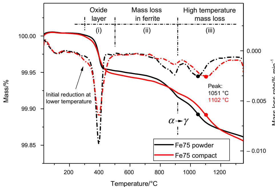
Fig. 4 TG/DTG curves of Fe75 powder and Fe75 compact at 10 °C min -1
