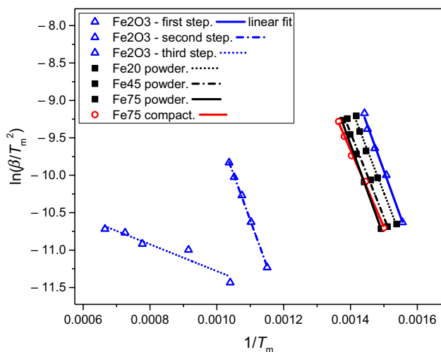
Fig. 7 Kinetic analyses of Fe 2 O 3 and oxide layer reduction
