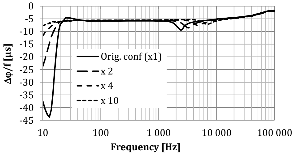
Figure 15: Phase angle error for different feed-back signal amplification, 10 Hz – 100 kHz for DUT 3.
