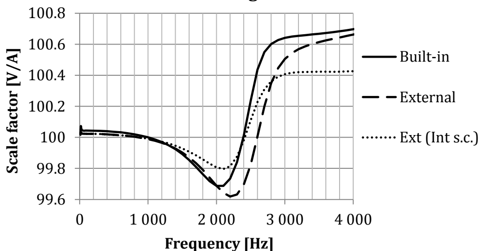
Figure 19: Zoom-in of the scale factor, SF for the DC- and the AC regions, 10 Hz to 4 kHz, for DUT 3 for the built-in shunt and the external shunt.
