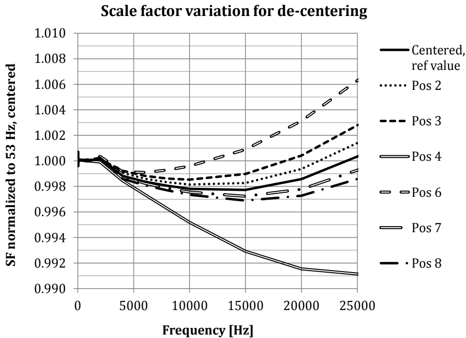
Figure 30: Normalized SF as a function of frequency for different de-centering positions.
