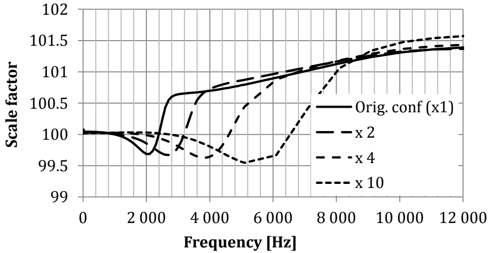
Figure 14: Scale factor for different feed-back signal amplification, 10 Hz – 12 kHz for DUT 3.
