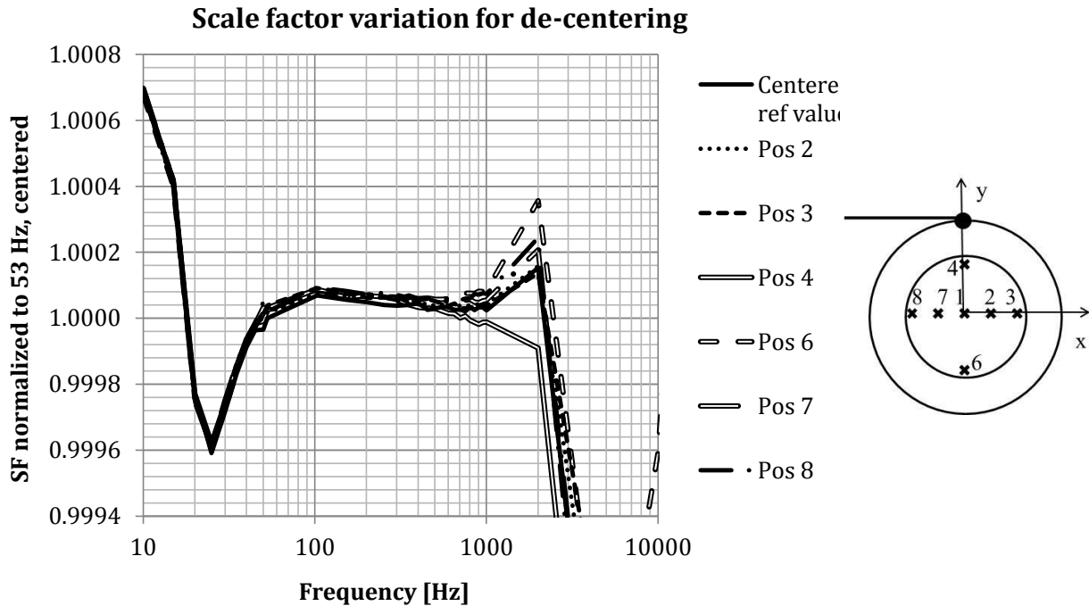
Figure 29: Left: Normalized SF as a function of frequency, 10 Hz – 10 kHz, for different de-centering positions. Right: Positions of primary conductor, Fig. 27a repeated.
