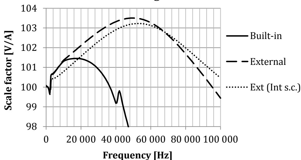
Figure 18: Zoom-in of the scale factor, SF for 10 Hz to 100 kHz for DUT 3 for the built-in shunt and the external shunt.
