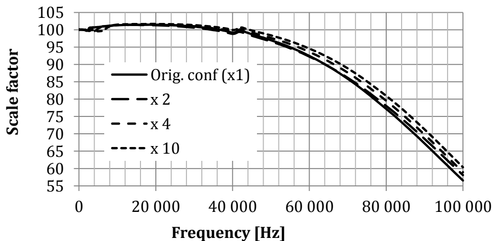
Figure 13: Scale factor for different feed-back signal amplification, 10 Hz – 100 kHz for DUT 3.
