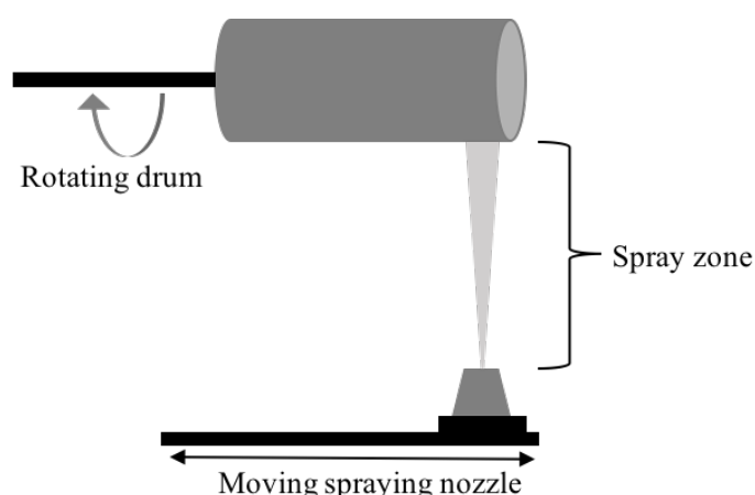
Figure 2. Schematic illustration of the manufacturing process of the model polymer films. The polymer solution was sprayed onto a rotating drum using a moving spraying nozzle.
