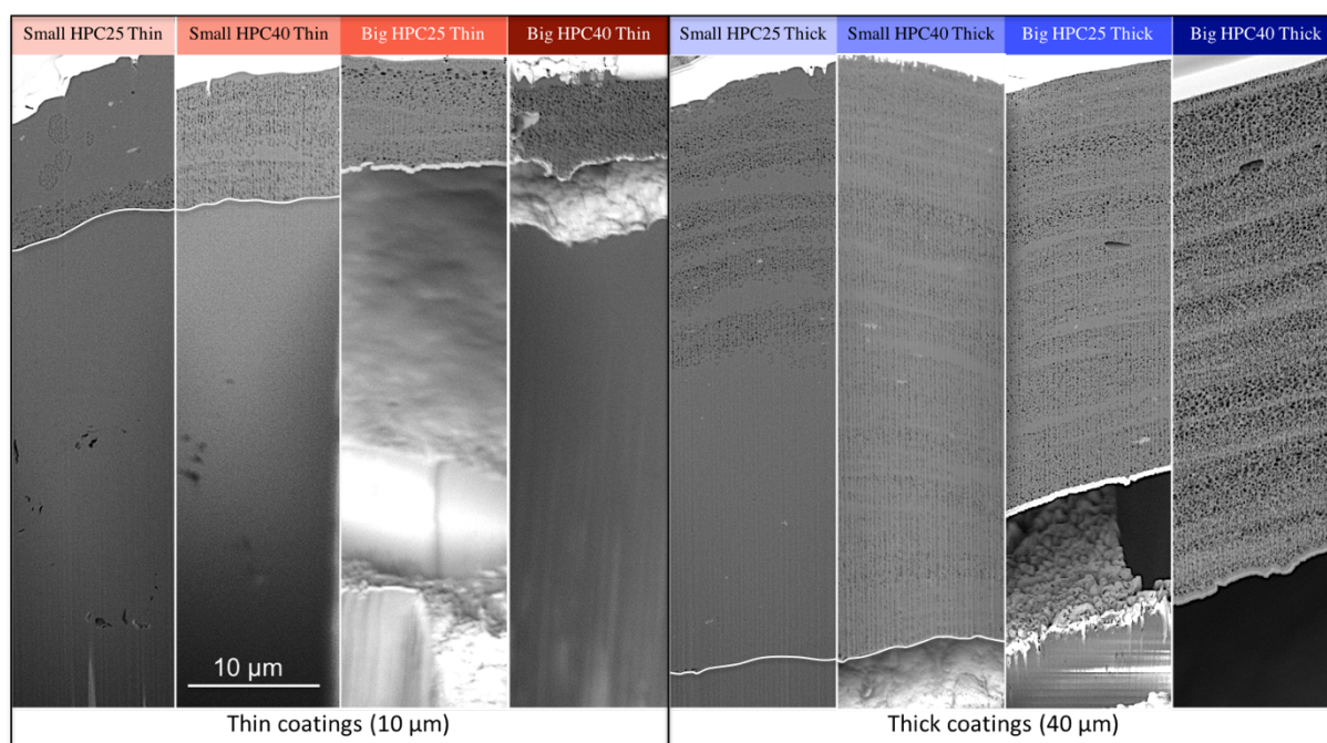
Figure 27. SEM BSE cross sectional images of pellets where thin coatings (10 μm) are seen on the left and thick coatings (40 μm) on the right.
