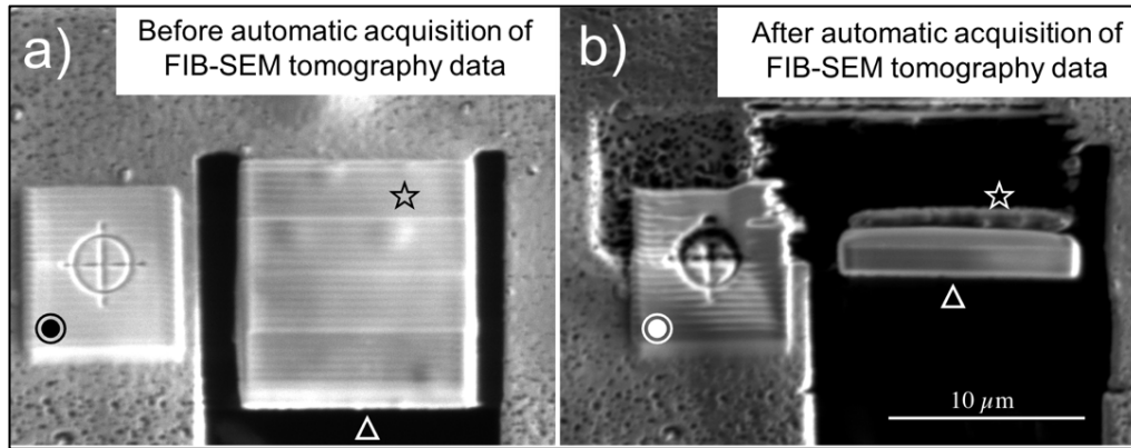
Figure 18. Ion beam SE images of the U shape when drift problem is observed where a) is before automatic acquisition of FIB-SEM tomography data and b) is after automatic acquisition of FIB-SEM tomography data.
