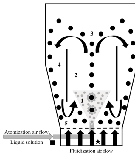
Figure 4. Schematic illustration of the Wurster coating process of pellets: 1) spray zone, 2) Wurster tube, 3) fountain region, 4) downbed region and 5) horizontal transport region.
