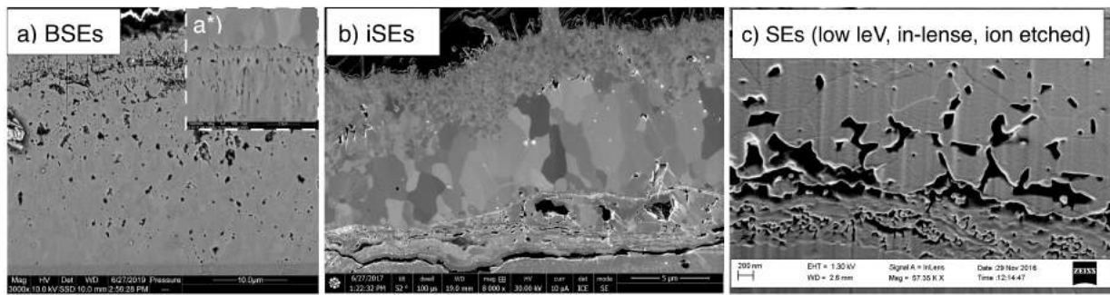
Figure 4.8: Examples of different imaging techniques to image oxide grains. a) BSE imaging (channeling contrast), b) iSE imaging (enhanced channeling contrast), c) low keV SE imaging on an ion-etched surface. The insert in a) ( a^* ) shows how an improved surface may enable for better grain contrast also in BSE mode.
