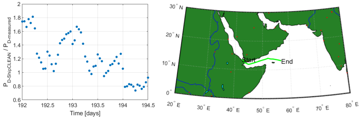
Figure 17: Position and power relation during two days for Ship 3.
