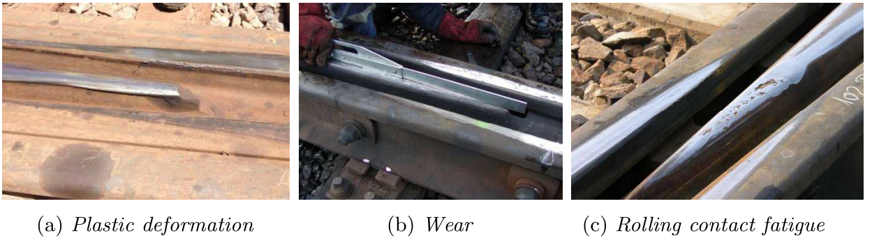
Figure 1.3: Three main damage mechanisms in S&C. Courtesy of voestalpine VAE GmbH.
