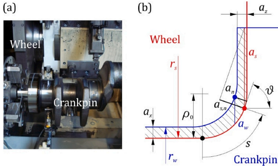
Fig. 7. (a) Crankpin grinding with (b) illustration and parameters.
