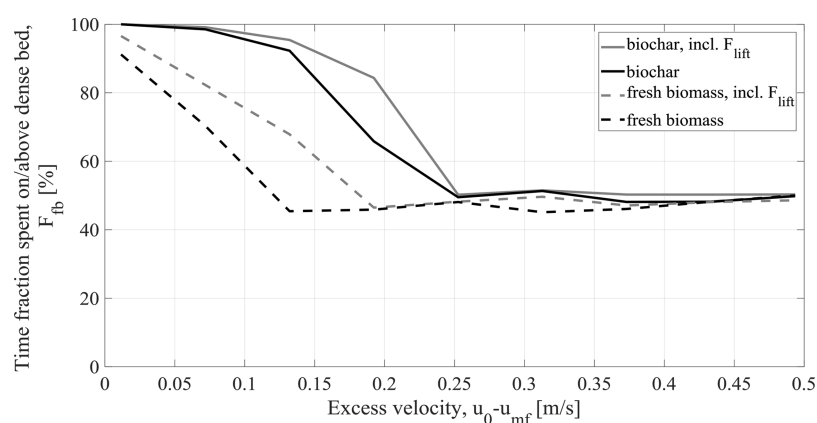
Figure 10. Modeled effect of the lift force on the time fraction that the fuel particles spend on and above the dense bed versus fluidization velocity. Fresh biomass and biochar, 4 cm in diameter, and \mu_e = 1.23 Pa s.
