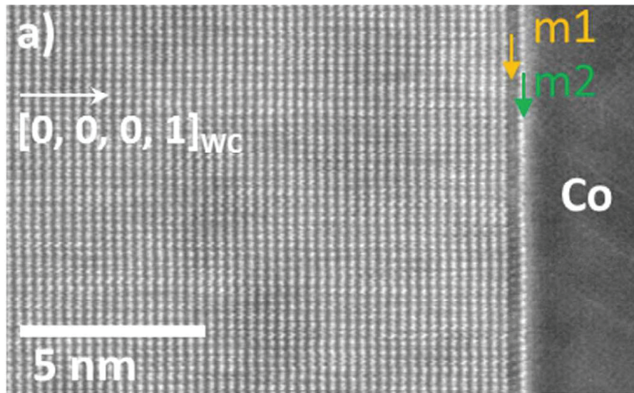
Figure 3.13: HRTEM image of a (Ti,W)C 1-x film in a TiC doped cemented carbide [110]. The film has a thickness of two metallic layers. Ti atoms are found to segregate to the first layer (m1) of the film, leaving one layer of W atoms (m2) towards Co.
