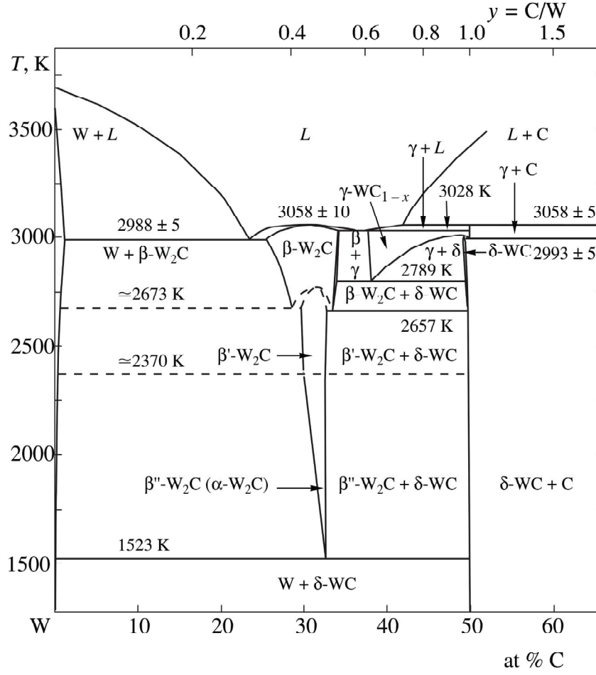
Figure 3.2: W-C phase diagram [60], where W denotes bcc W, C denotes graphite, \beta^* - W_2C denotes various tungsten semicarbides, \delta -WC denotes hexagonal WC and \gamma -WC denotes cubic WC.
