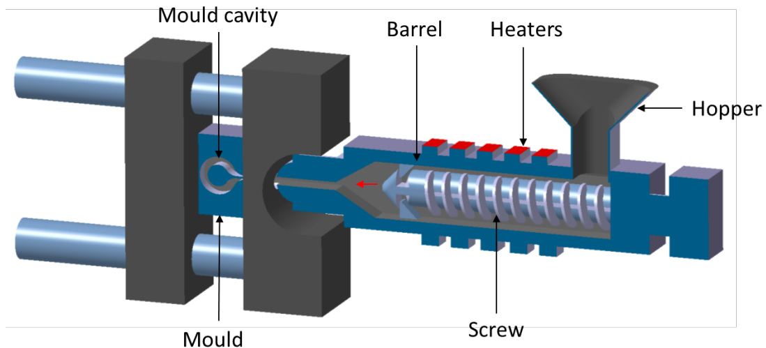
Figure 6: Illustration of Injection molding process
