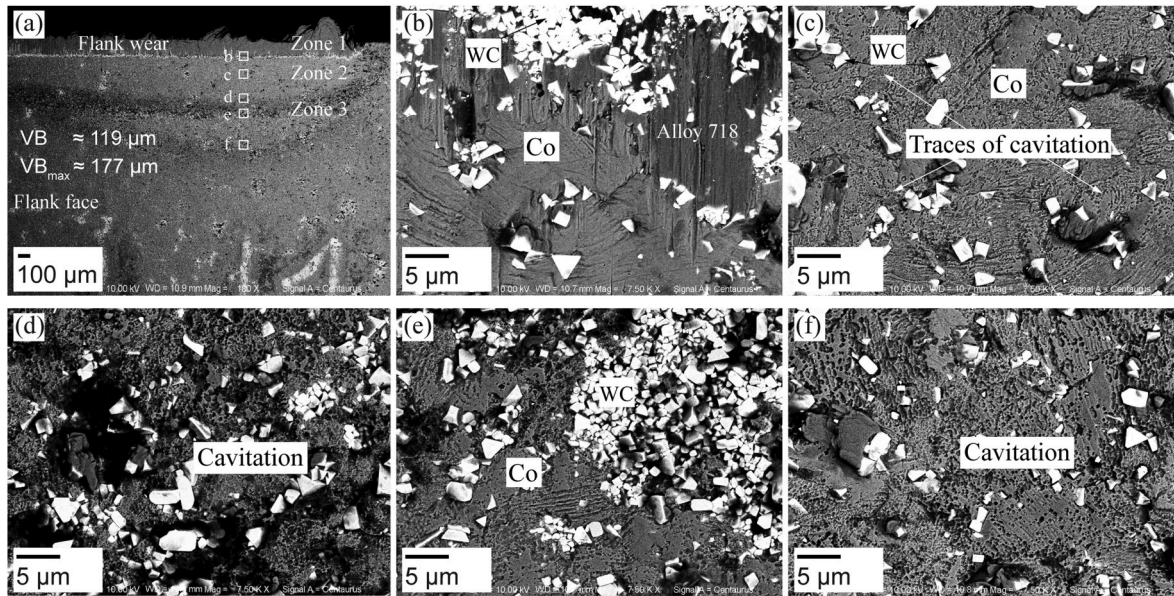
Fig. 7. BSE micrographs of Tool-1 machined Alloy 718 at v_c 45 m/min, f_n 0.2, rake pressure 16 MPa and flank pressure 4 MPa: (a) flank face illustrating 3 different zones; selected areas on higher magnification: (b) border of Zone 1 and 2, (c) Zone 2, (d) border of Zone 2 and 3, (e) Zone 3, and (f) further away from Zone 3.
