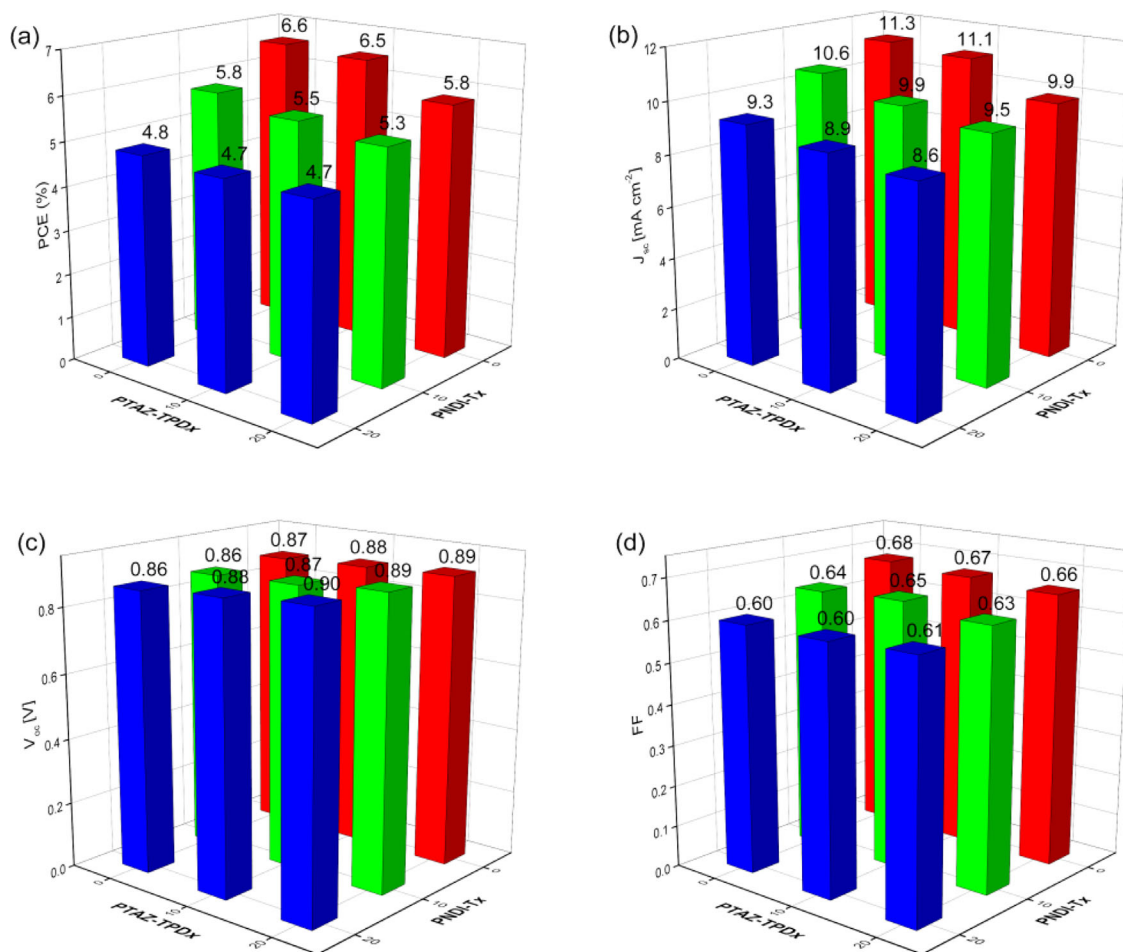
Figure 2. Photovoltaic parameters of the optimized PTAZ-TPD x :PNDI-T x solar cells acquired under AM1.5G illumination (100 mW cm -2 ): a) PCE, b) J sc , c) V oc , and d) FF.
