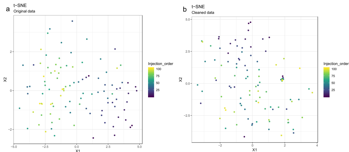
Figure 9. The drift pattern in the injection order (the color trend) using the t-distributed stochastic neighbor embedding (t-SNE) method is visible before drift correction (a), whereas after drift correction (b), the samples are more randomly scattered.
