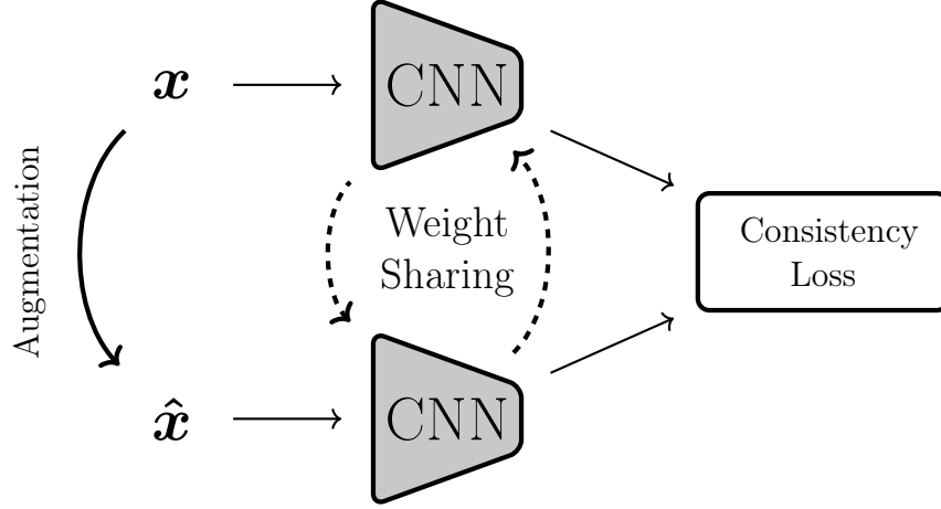
Figure 2.5: A consistency regularization training schematic for semi-supervised learning. The network is trained to produce consistent output for the original input, x , and an augmented version of the image, \hat{x} . The assumption made is that the augmentation should not change the labels.
