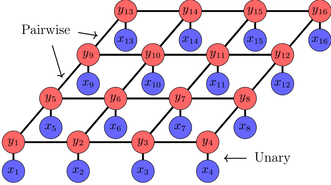
Figure 2.4: CRF with a simple nearest neighbour connectivity, neighbourhood size four. The variables y_u are assigned class labels while the variables x_u represents the pixel values.
