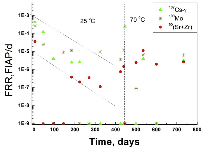
Fig. 12. Autoclave 5U1. \text{FRR}(t) (FIAP/day) for Cs measured by \gamma -spectrometry, Sr and Mo. Negative values of FRR for a given interval are plotted on the x-axis.
