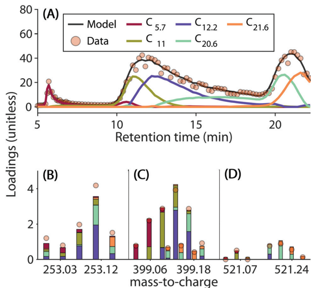
Fig. 2 Comparison of measured and modelled data (sample location Lat/Lon: 57.133471°N/15.533230°W). (A) Measured vs. modelled chromatogram (sum of all formulas). Coloured lines refer to the intensities of five PARAFAC components. (B–D): Measured vs. modelled molecular formulas in three different mass-to-charge ranges (identical intensity scale). The coloured lines in (A) and bars in (B) indicate the contribution of each component to the total modelled signal.
