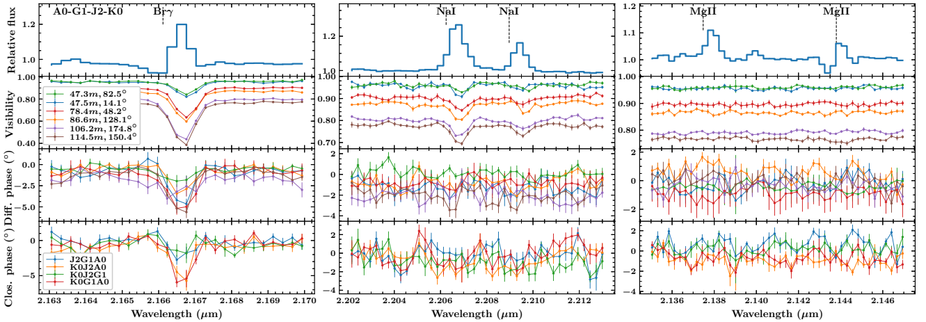
Fig. 7. Representative example of relative flux, visibility, differential, and closure phase as a function of wavelength around the Bry and NaI doublet emission towards IRAS 17163 using GRAVITY on the large configuration. The 6 baselines and 4 triplets of A0-G1-J2-K0 configuration are plotted with different colours. Both Bry emission and NaI show a smaller visibility than the continuum while Bry shows a larger drop. Mg II does not show changes in visibility or phases. A differential phase change is also detected towards Bry but not towards Na I.
