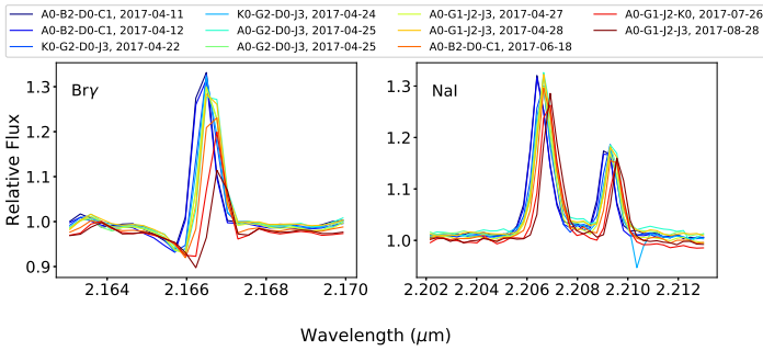
Fig. 3. Spectra of the Bry ( left ) and Na I ( right ), normalised to the continuum level, for the different observing dates and configurations in different colours. The dataset shows a gradual drop in the flux of the Bry emission (up to \sim 67\% ) over the observing period of four months, while Na I emission does not vary significantly.
