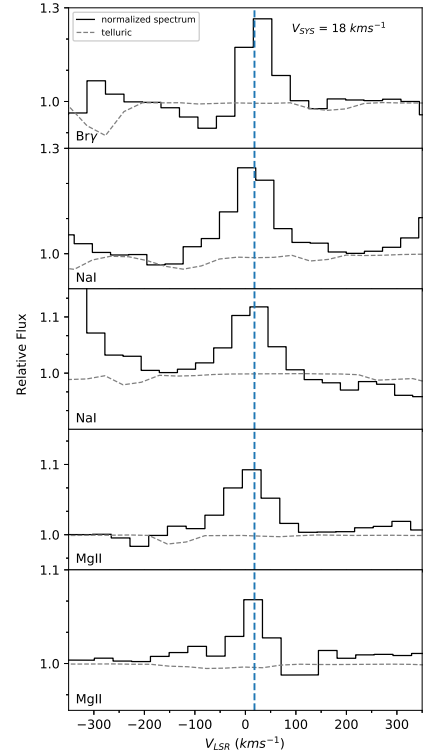
Fig. 4. Line profiles of the observed Bry, Na I, and Mg II emission towards IRAS 17163. The dotted line represents the telluric absorption spectrum applied to correct the spectrum of the object. The vertical line represents the systemic velocity as reported by Wallström et al. (2015) using the optical Fe II emission.
