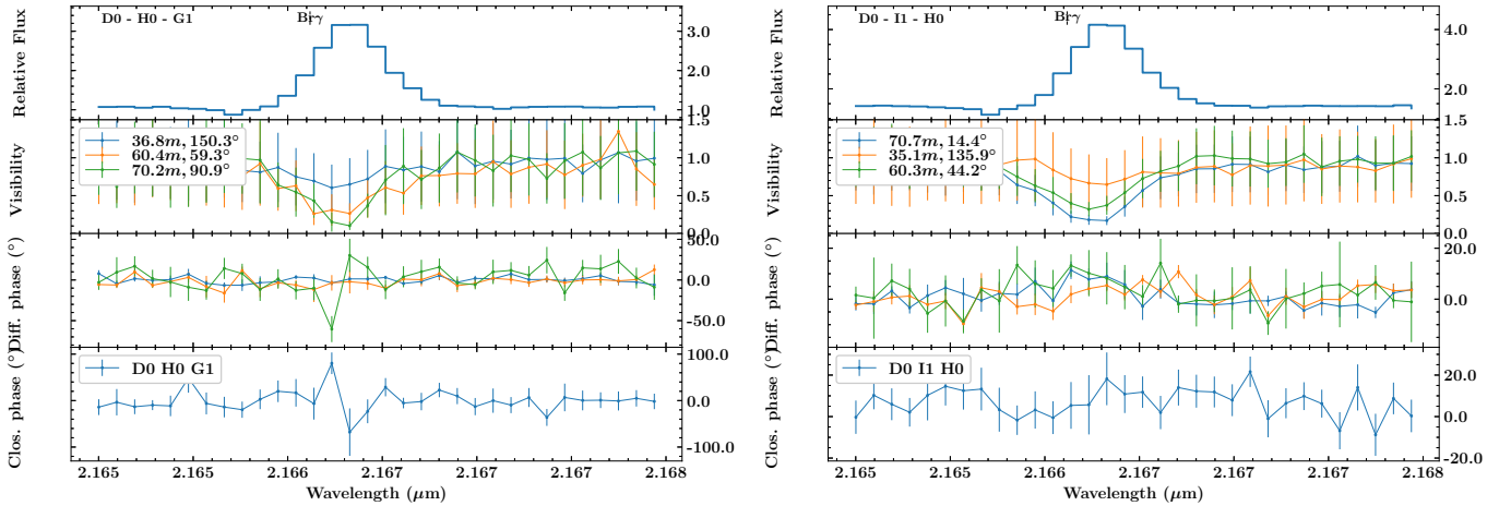
Fig. 8. Representative examples of relative flux, visibility, differential, and closure phase as a function of wavelength for the AMBER D0-H0-G1 and D0-I1-H0 configurations around the Bry emission towards IRAS 17163.
