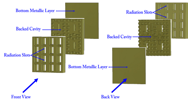
FIGURE 3. Exploded views for the 4 × 4-Element sub-array. Left-side: front view, and Right-side: back-view.
