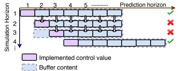
Fig. 3. Buffer implementation: The use of control data stored in the buffer when new control data is not received is illustrated.
