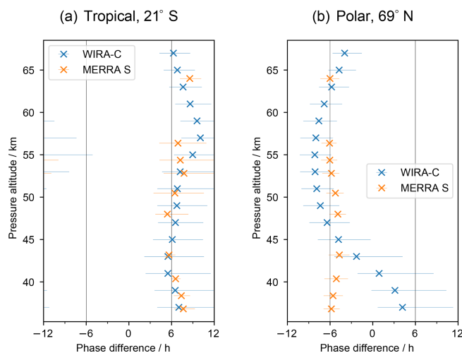
Figure 4. Phase difference between meridional and zonal diurnal wind tide ( \Delta\phi = \phi_{\text{merid.}} - \phi_{\text{zonal}} ) for the tropical and arctic campaigns in WIRA-C measurements and the MERRA-2 reanalysis.
