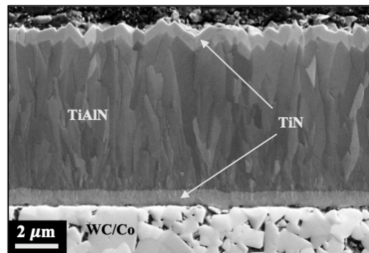
Figure 3.1. Cross section micrograph of a CVD TiN-TiAlN-TiN multi-layered coating deposited onto a cemented carbide substrate. The image was acquired using a scanning electron microscope.
