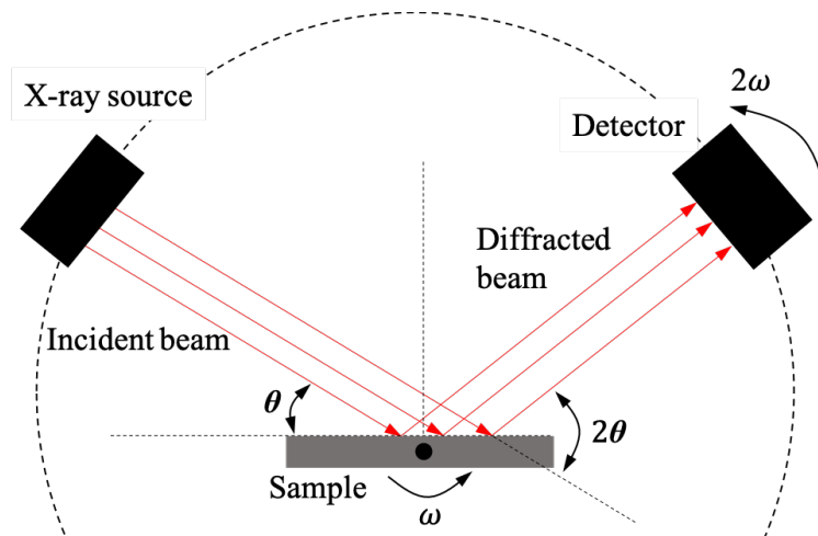
Figure 4.1. Schematic illustration of an X-ray spectrometer for a \theta - 2\theta scan.
