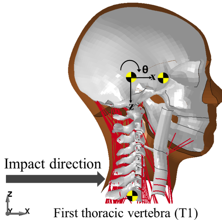
Figure 3.5 Simulation Setup
