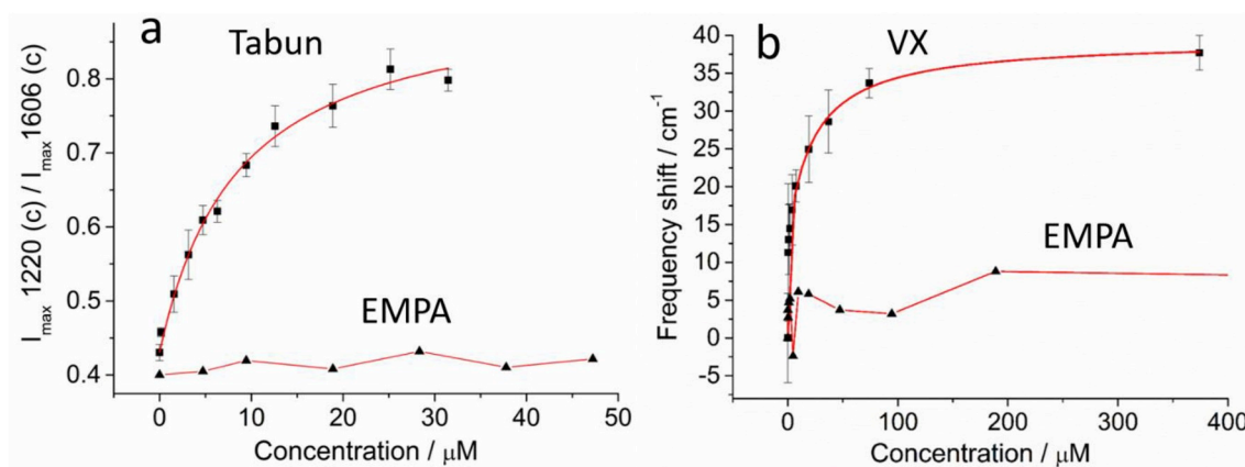
Fig. 4. Adsorption isotherms for Tabun and VX obtained in drop-and-dry experiments. Intensity rise at 1220\text{ cm}^{-1} for Tabun is fitted with one binding site approximation ( K_d = 8.5 \pm 0.91\ \mu\text{M} , R^2 = 0.99 ) whereas spectral shift at 945\text{ cm}^{-1} for VX needs two binding sites approximation ( K_{d1} = 0.09 \pm 0.03\ \mu\text{M} , K_{d2} = 23.9 \pm 2.44\ \mu\text{M} , R^2 = 0.99 ). No spectral trend was seen for control substance EMPA.
