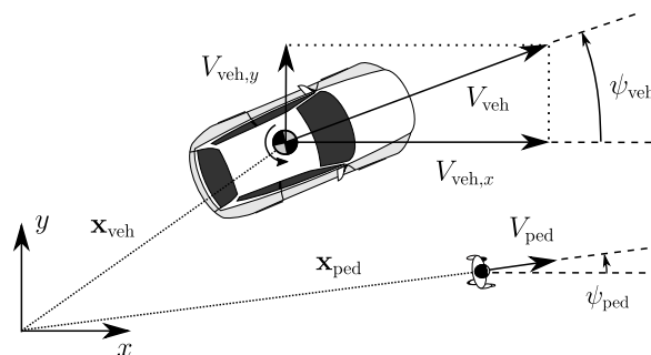
Fig. 2. Vehicle and pedestrian kinematic variables in the global frame.
