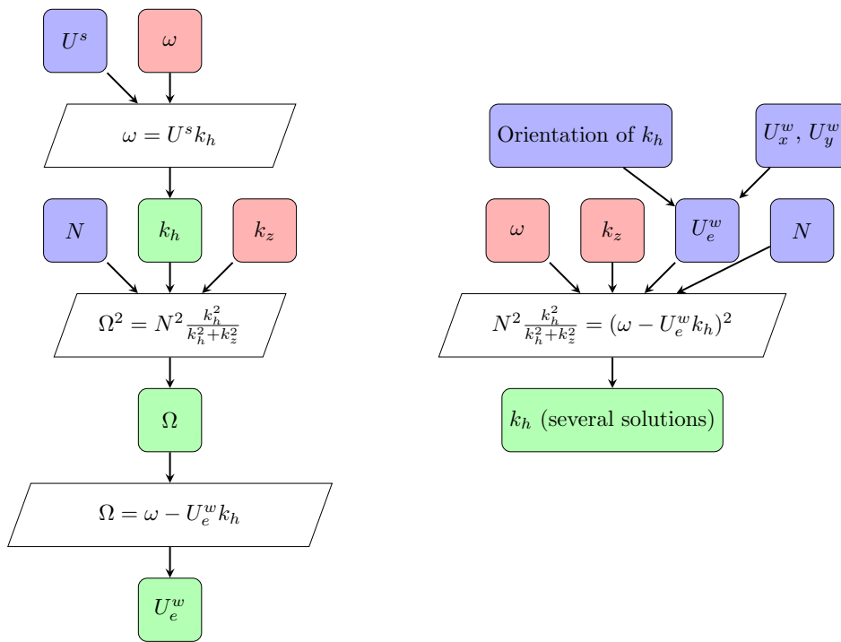
Figure 2.5: Frameworks for ground-based lidar observations. Observed wave properties are coloured in red, calculated properties are in green and additional information in blue. The left panel shows when U^s is known. The right panel shows when U_e^w is known and the resulting horizontal wavelength may be up to 4 real solutions due to the quartic function.
