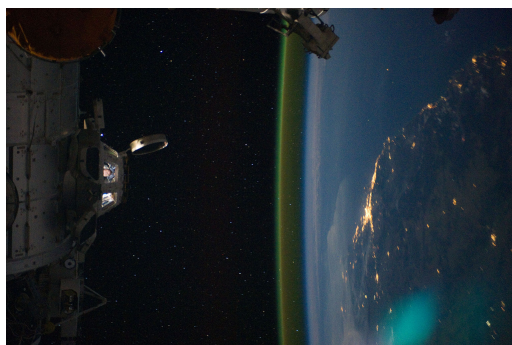
Figure 3.1: Airglow above the horizon captured from the International Space Station. Image from NASA.
