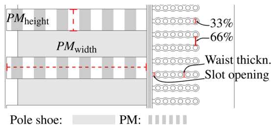
FIG. 2. Geometry and definitions of the model. Height is defined in the direction of PM magnetization.
