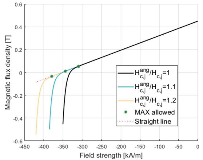
FIG. 7. Demagnetization curves for different H_{c,j}^{\text{ang}} . The straight dotted lines depict (1) used in Comsol. The asterisks (*) represent the positions where the exponential function starts to deviate from the straight line.
