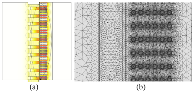
FIG. 3. (a) The geometric mapping and (b) an example of the mesh.
