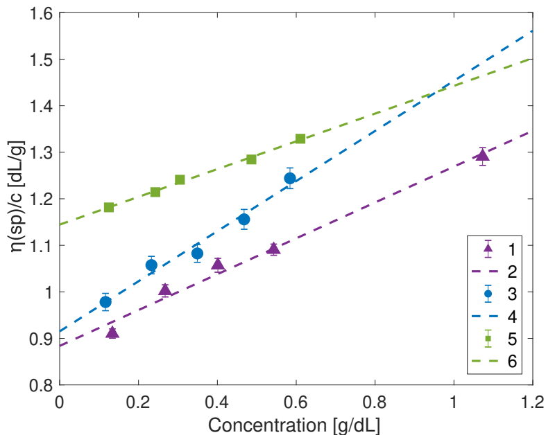
Figure 5.7: Specific viscosity divided by concentration ( \eta_{sp}/c ) as a function of cellulose concentration, used to extrapolate(see trendlines 2, 4 and 6) values of intrinsic viscosity at 25 °C for MCC dissolved in 4 mol%: NaOH(aq) (1), TMAH(aq) (3), and 50/50 NaOH/TMAH(aq) (5)
