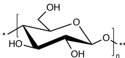
Figure 2.1: The structure of the repeating unit of cellulose, the anhydroglucose unit
