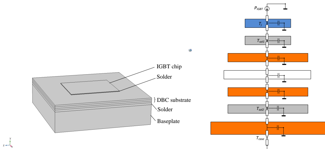
(a) IGBT chip with euqivalent area of substrate and (b) A 2D Caer thermal impedance network of one IGBT chip
