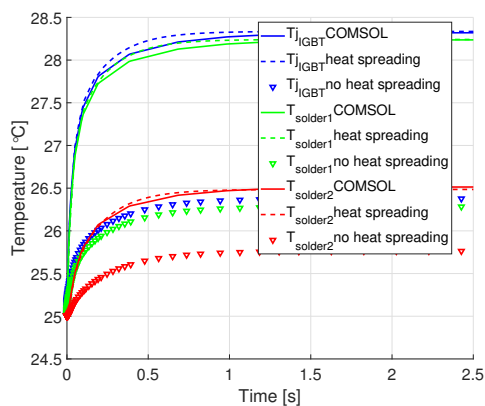
Fig. 8: Simulation results comparison with considering heat spreading effect
